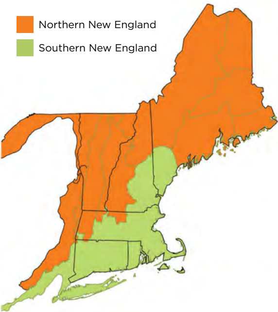
The above map illustrates the demarcation of northern and southern New England used in Table 1 based on ecological subsections. Northern New England includes ecological subsections M211A, B, C, and D, and M211E and J. Southern New England includes ecological subsection M221A.
