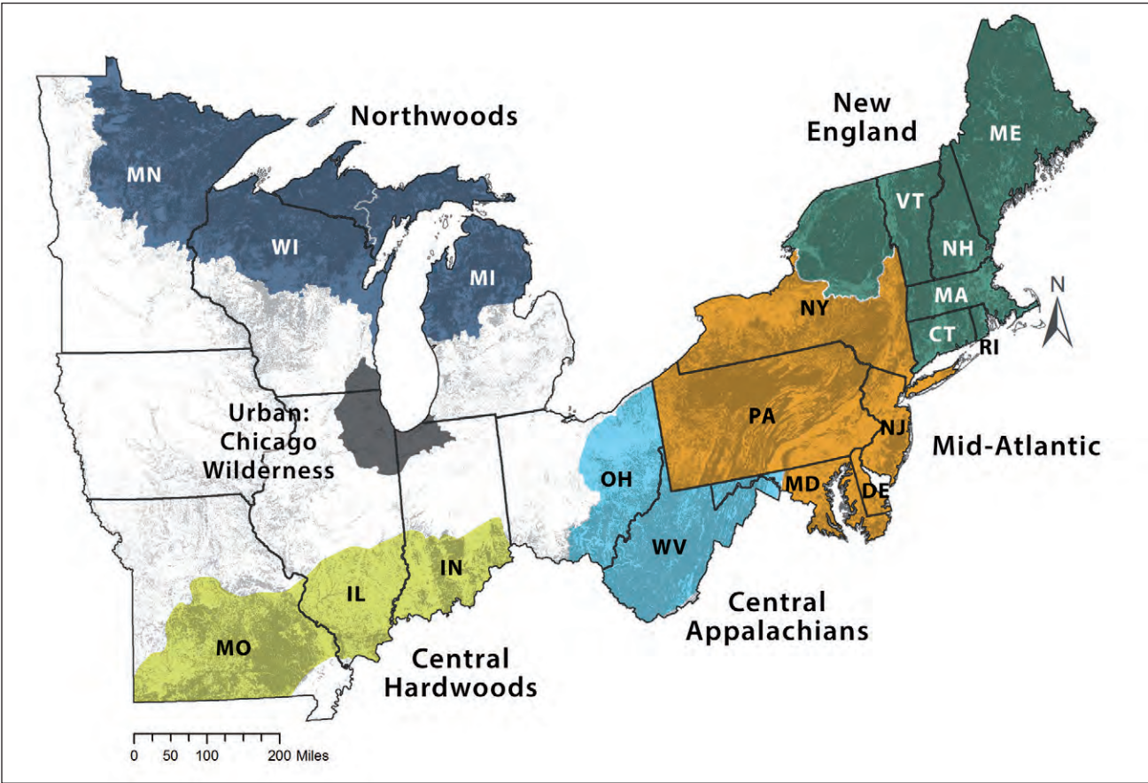
Figure 2.—Climate Change Response Framework ecoregional project areas.
