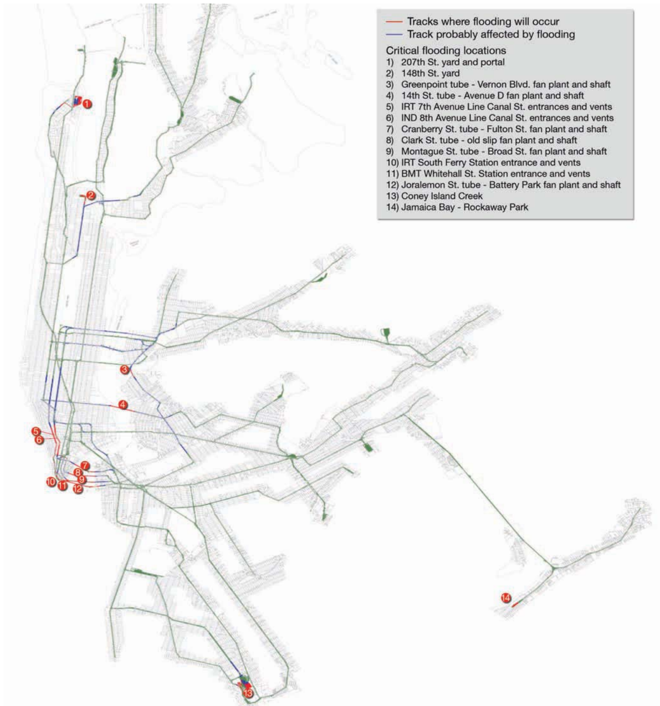
Figure 9.14 MTA subway flooding map for a category-1 hurricane based on surge heights listed in USACE (1995)
