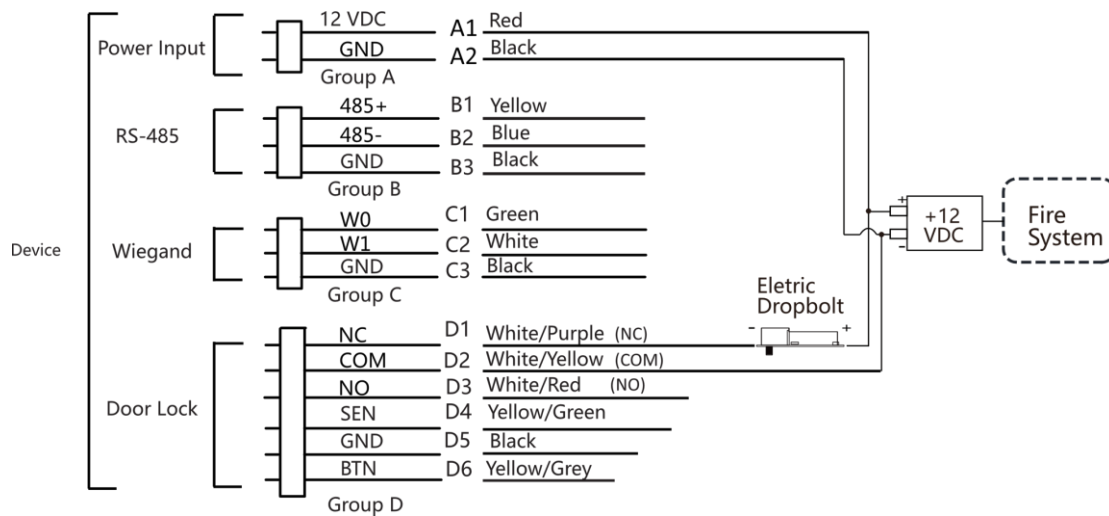
Figure 4-3 Wire Device
