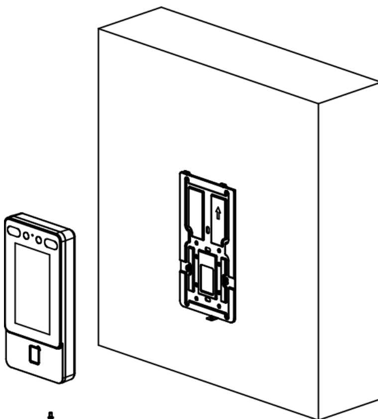
Figure 3-8 Hang Device
