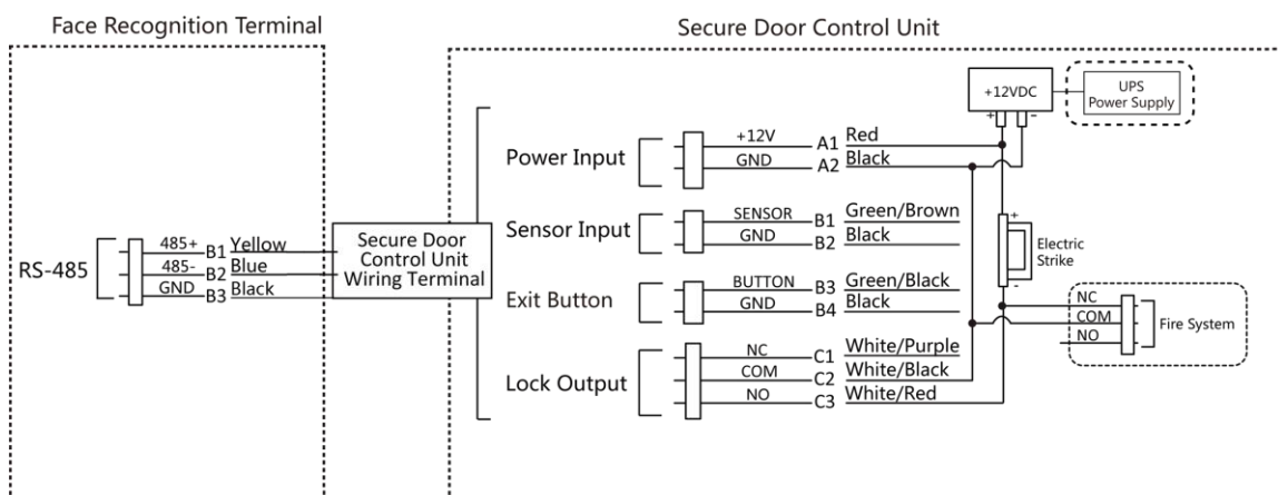
Figure 4-8 Wiring Diagram
