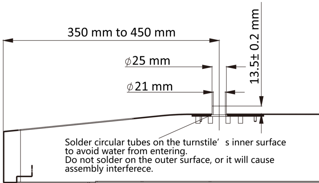
Figure 3-17 Solder Tubes
