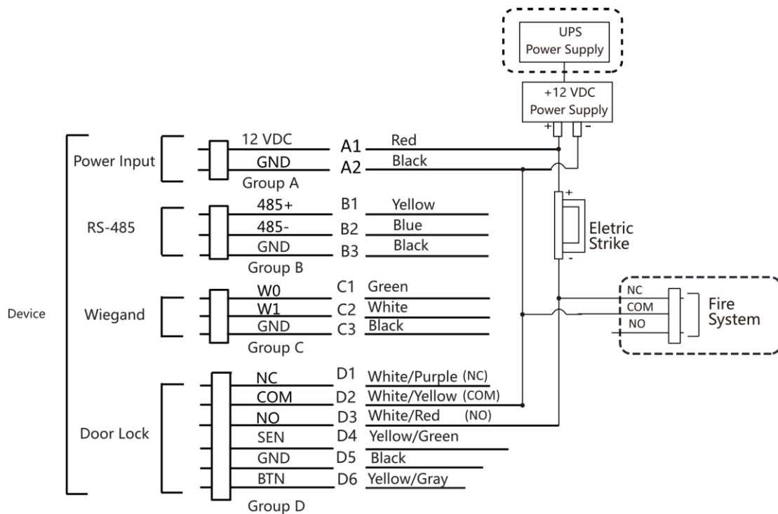
Figure 4-7 Device Wiring
