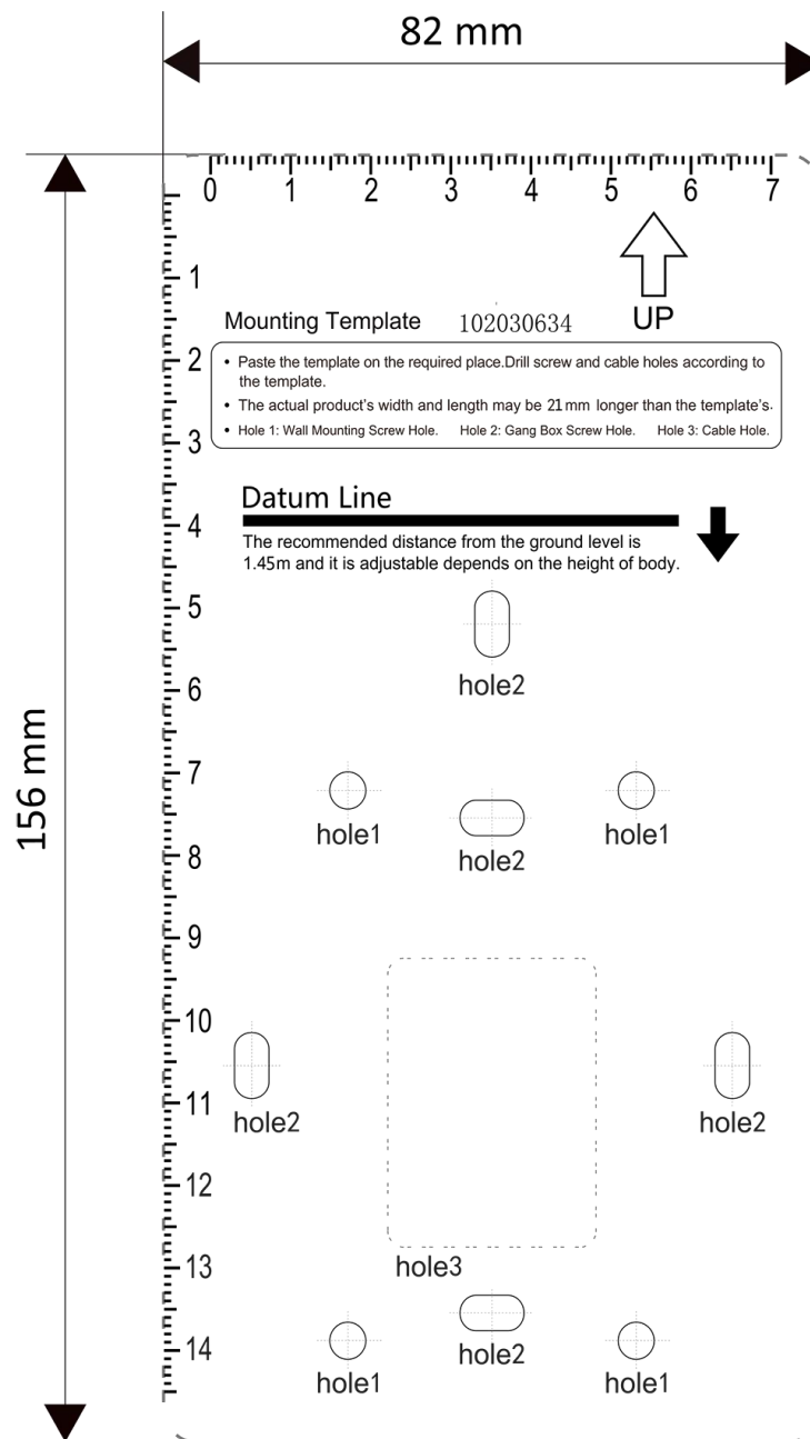
Figure 3-5 Mounting Template
