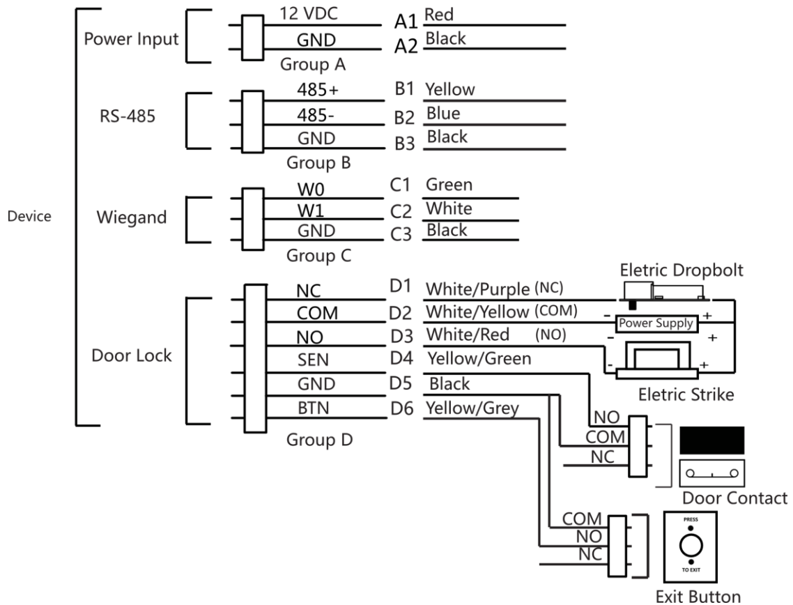
Figure 4-1 Device Wiring
