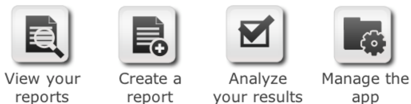
Figure 3.1. Getting Started
