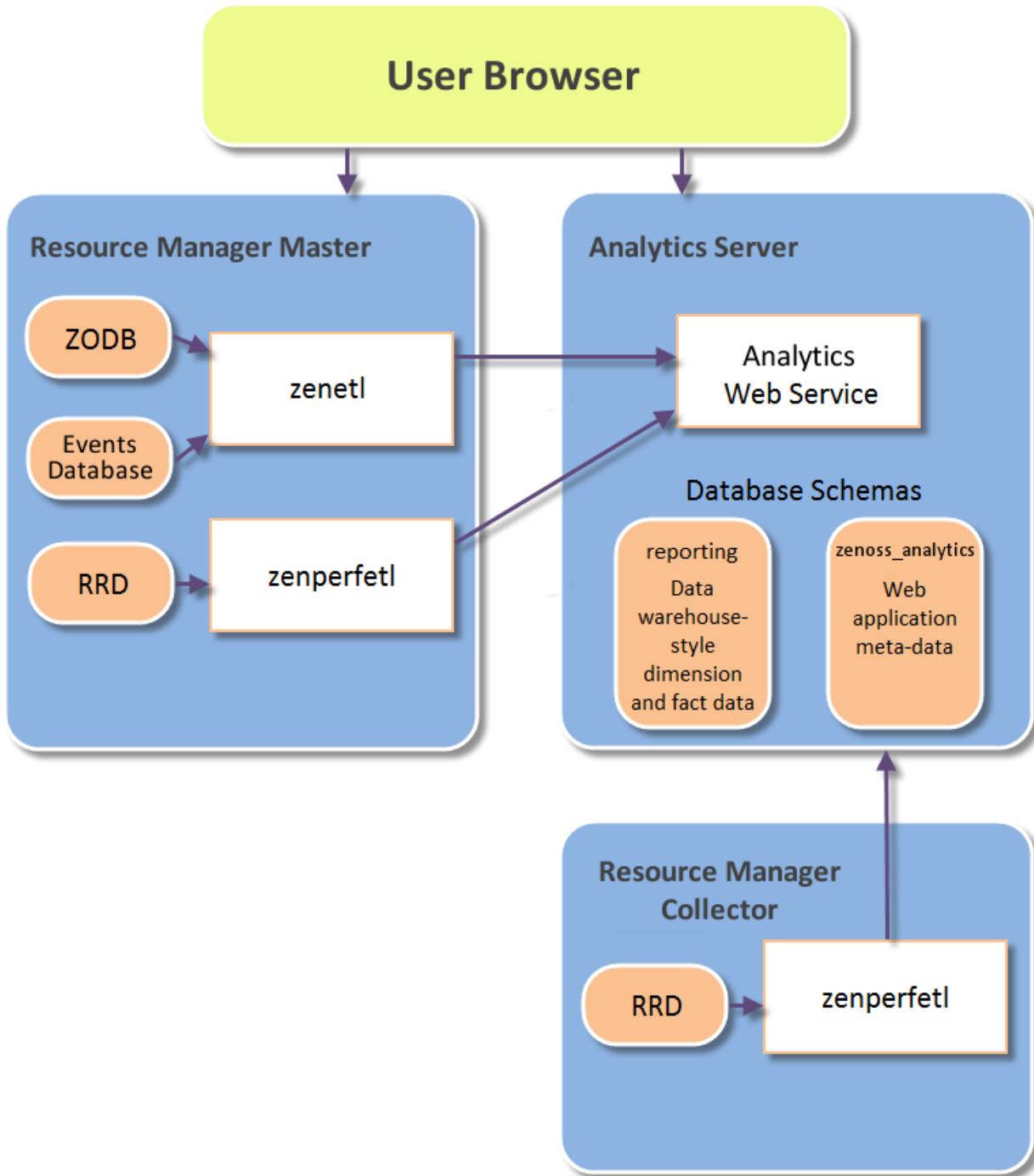
Figure 1.1. Analytics Components
