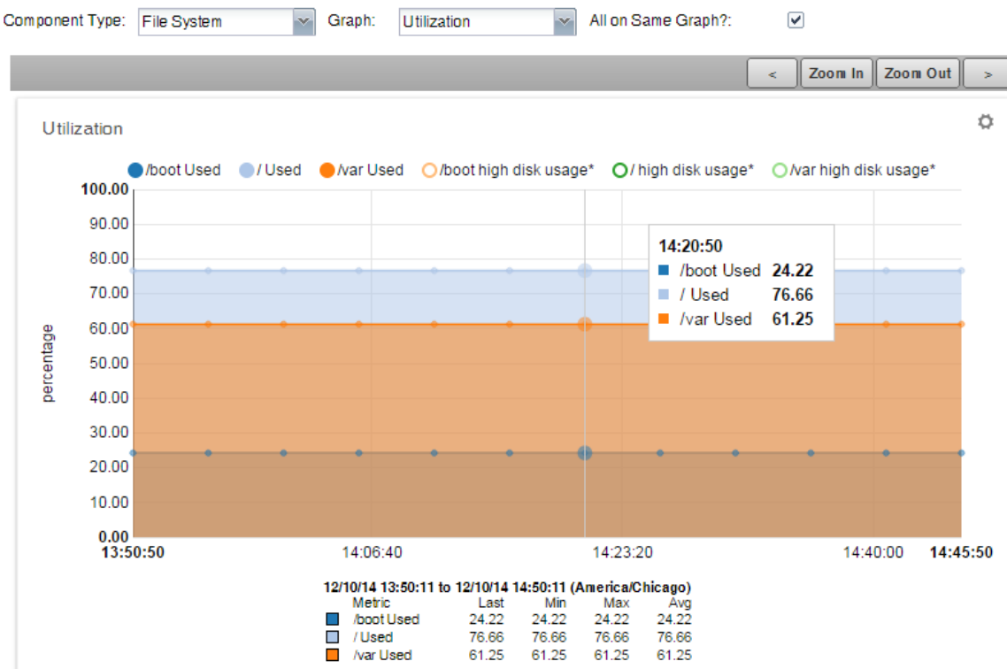
Figure 39: Component Graph (Device)
