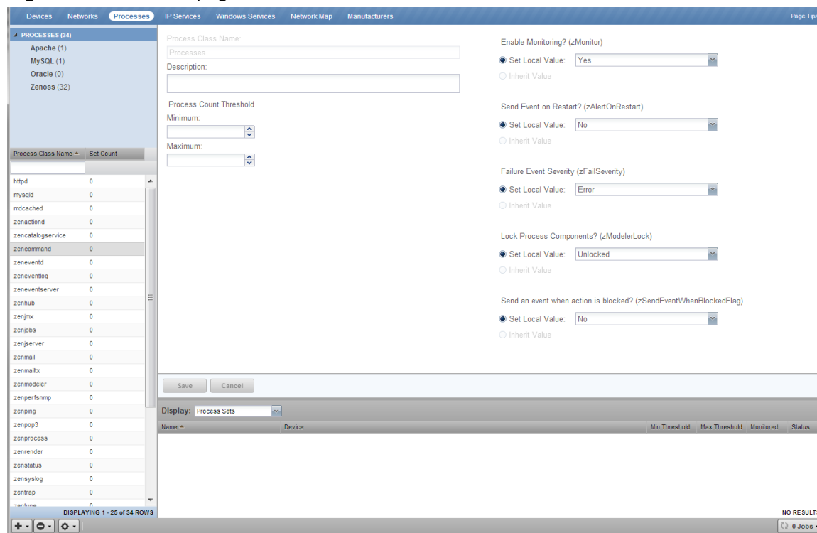
Figure 55: Processes page
