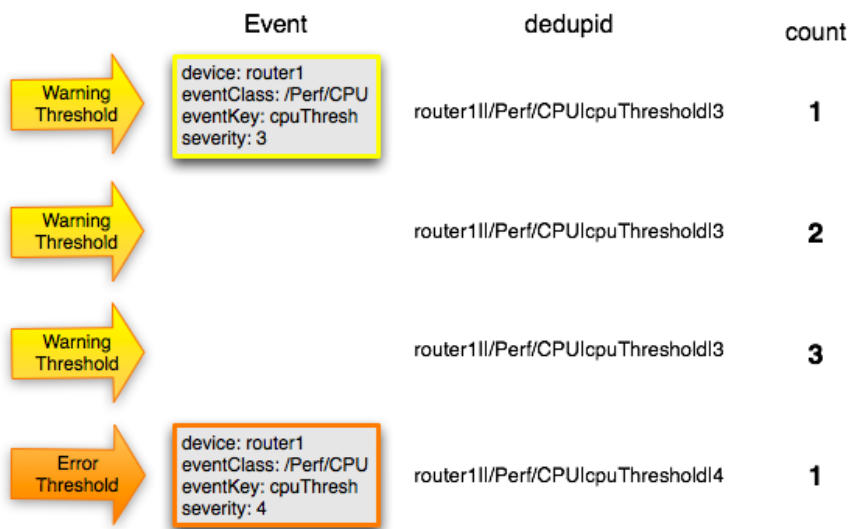
Figure 73: Event De-Duplication
