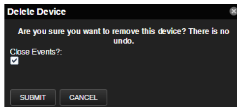
Figure 47: Delete Device
