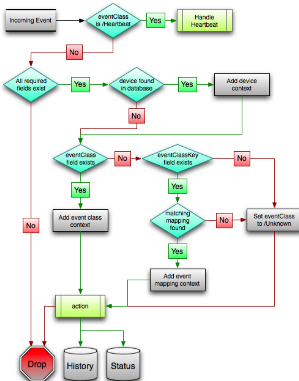
Figure 82: Event Processing
