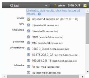
Figure 11: Search Results
