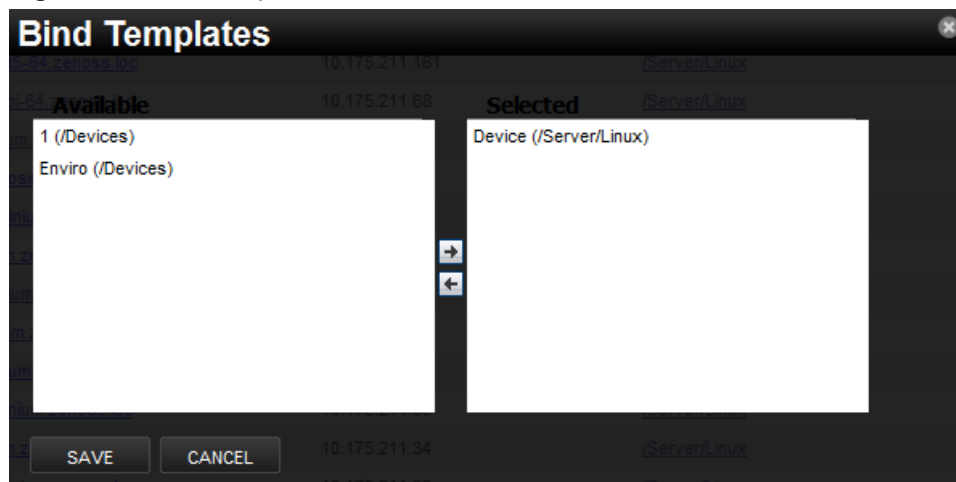
Figure 54: Bind Templates
