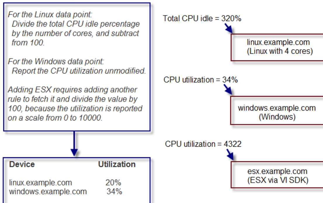
Figure 67: CPU Utilization Report
