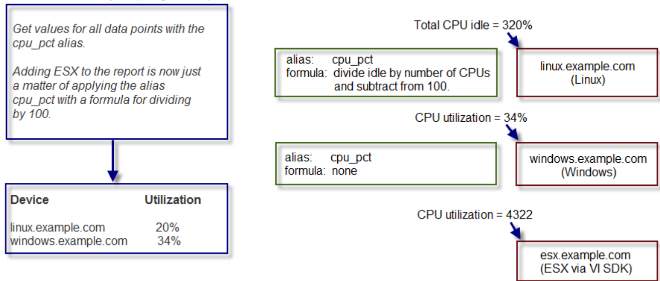
Figure 68: Alias-Based CPU Utilization Report
