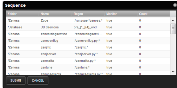
Figure 59: Sequence dialog
