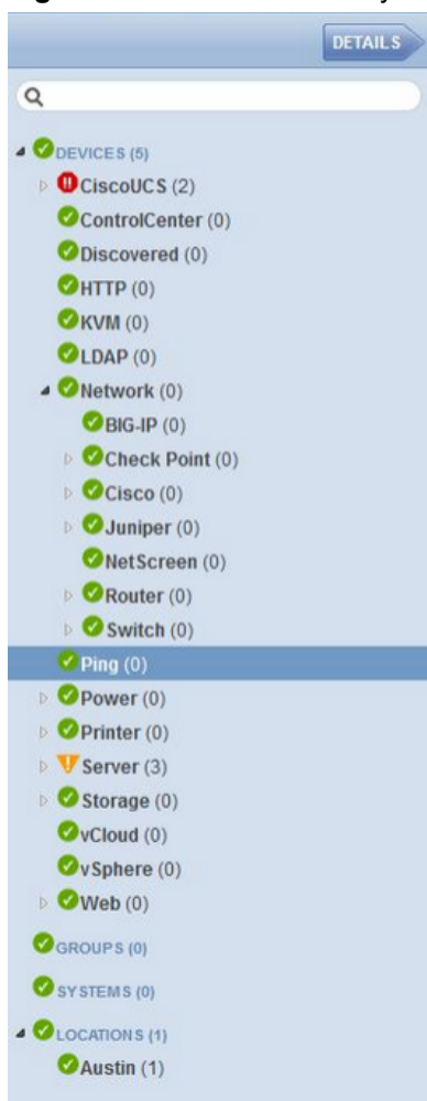
Figure 87: Devices Hierarchy
