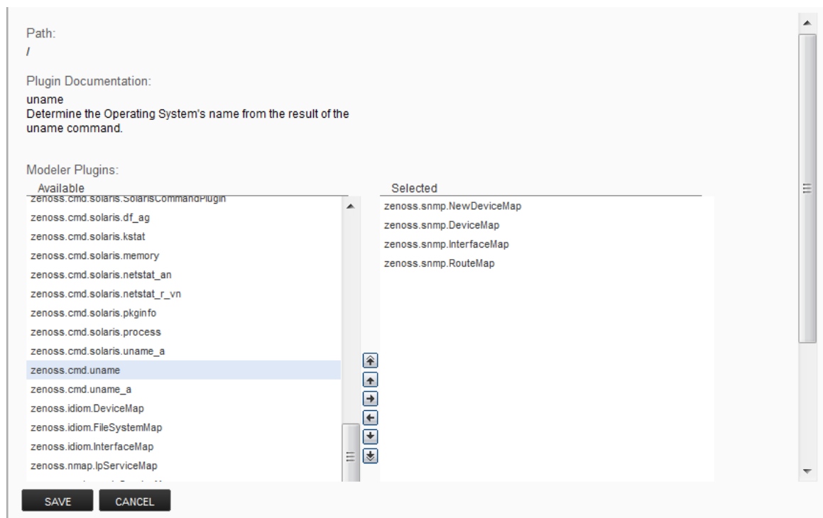
Figure 34: Add Plugin
