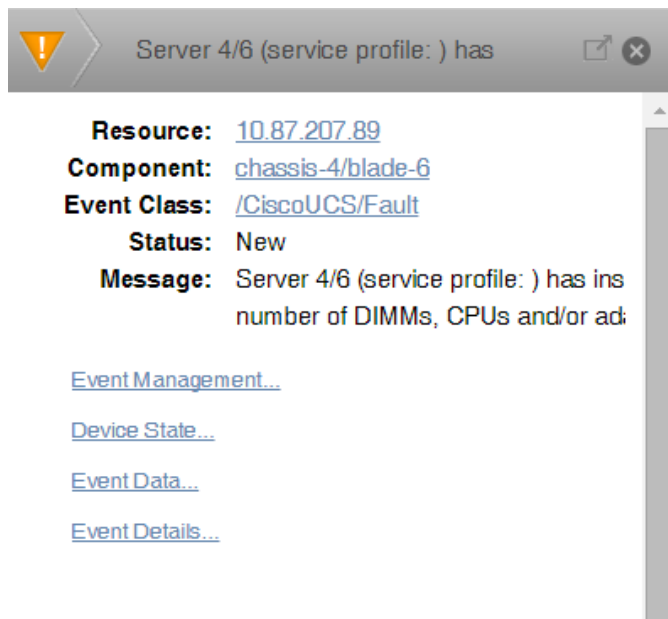
Figure 80: Event Details
