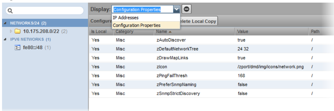
Figure 53: Networks
