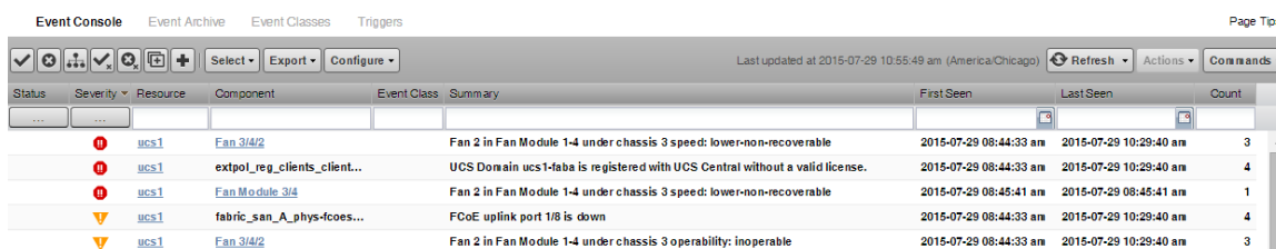
Figure 13: Event Console
