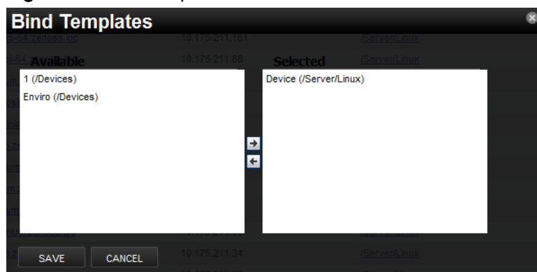
Figure 66: Bind Templates
