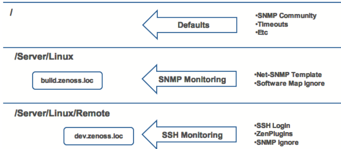
Figure 91: Device Class Tree and Inheritance
