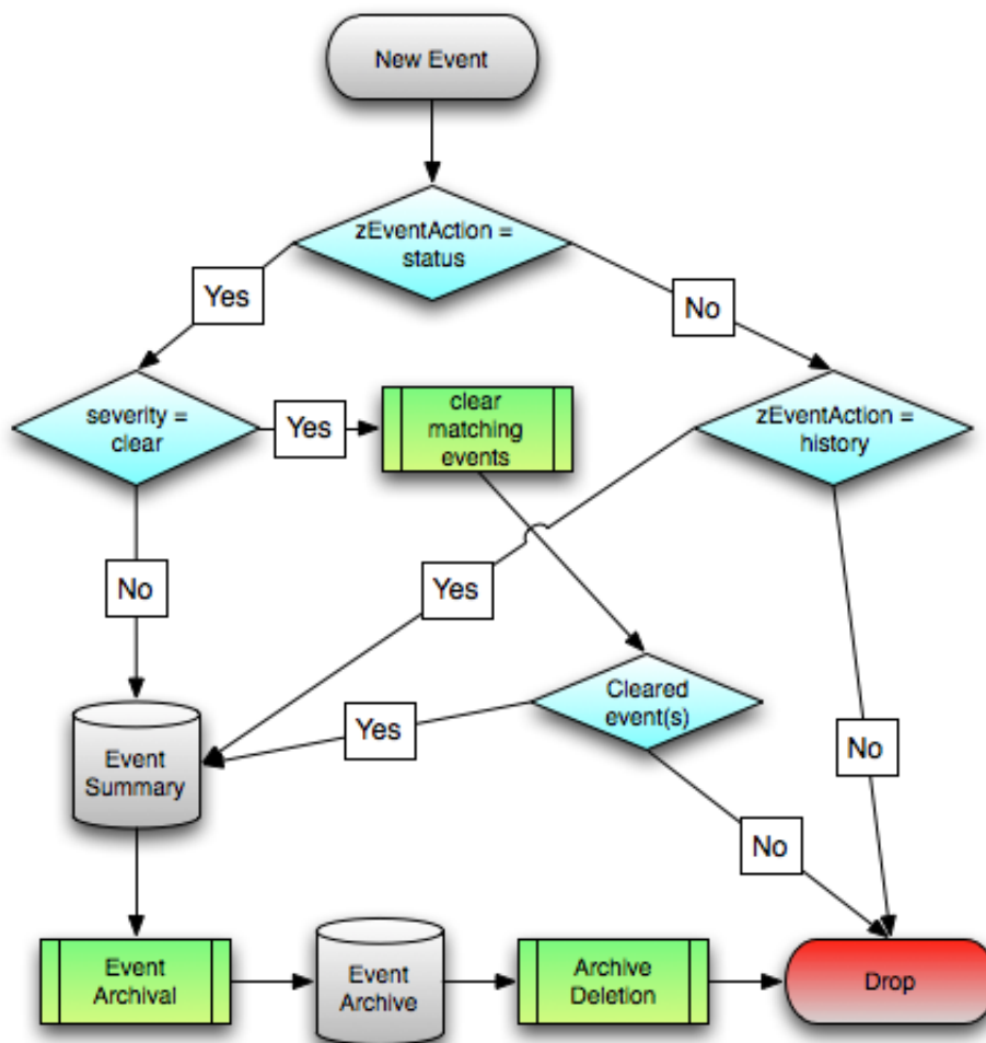
Figure 83: Event Life Cycle
