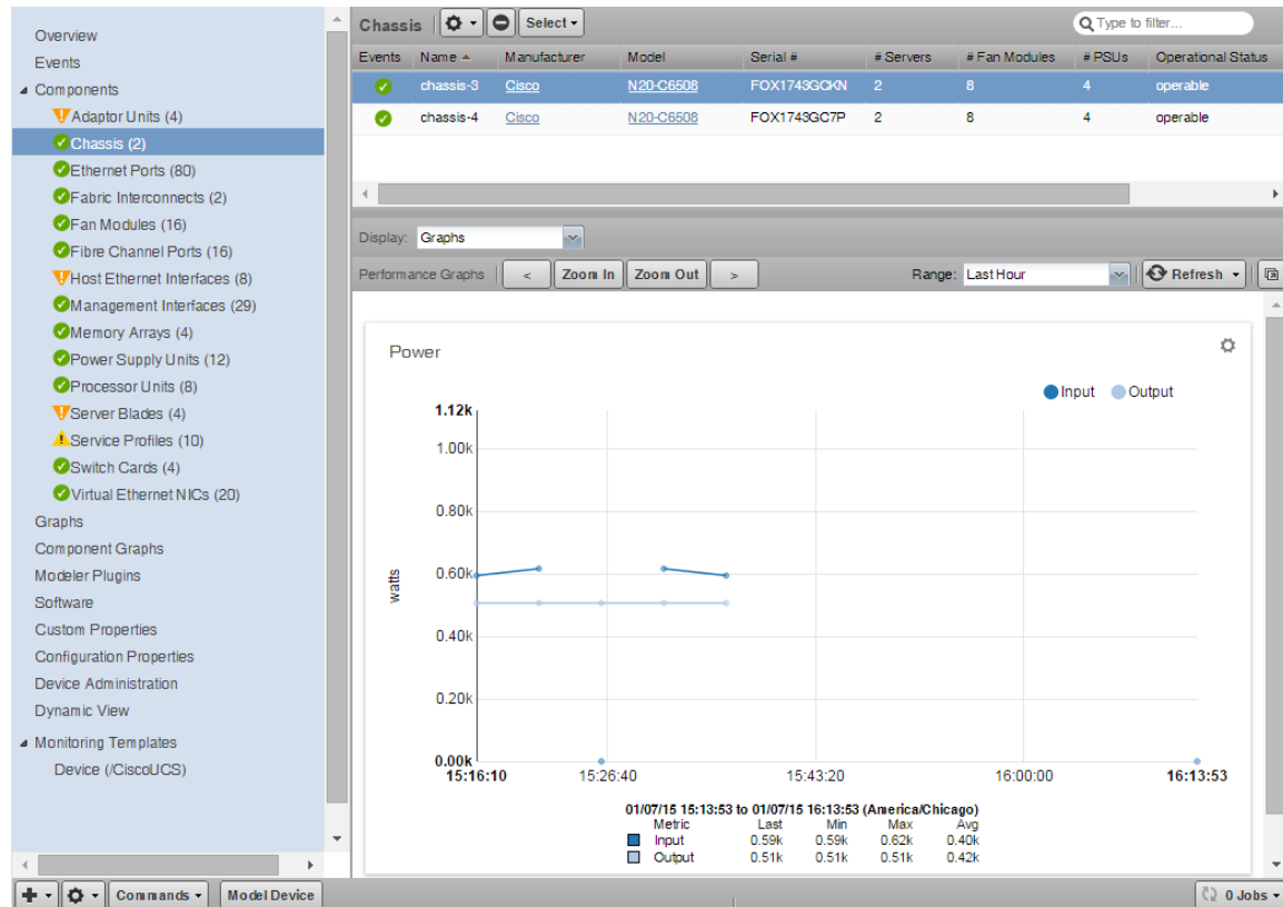
Figure 37: Device (Components)
