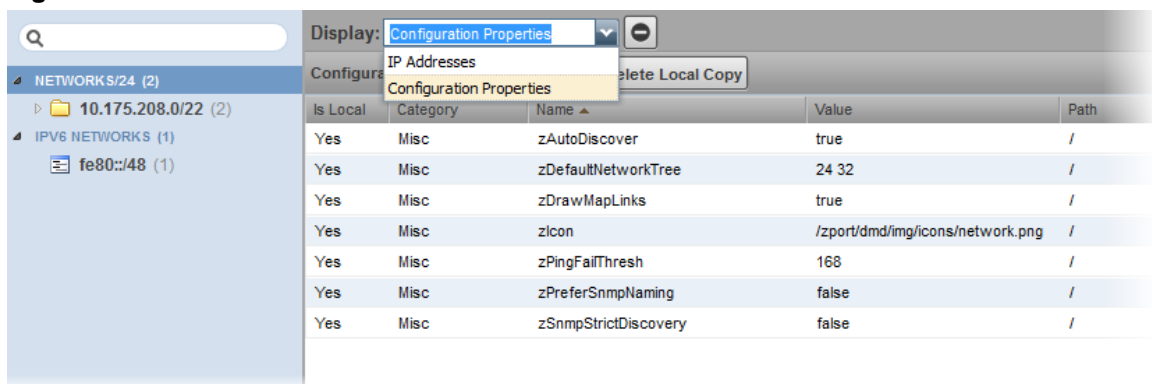
Figure 50: Networks
