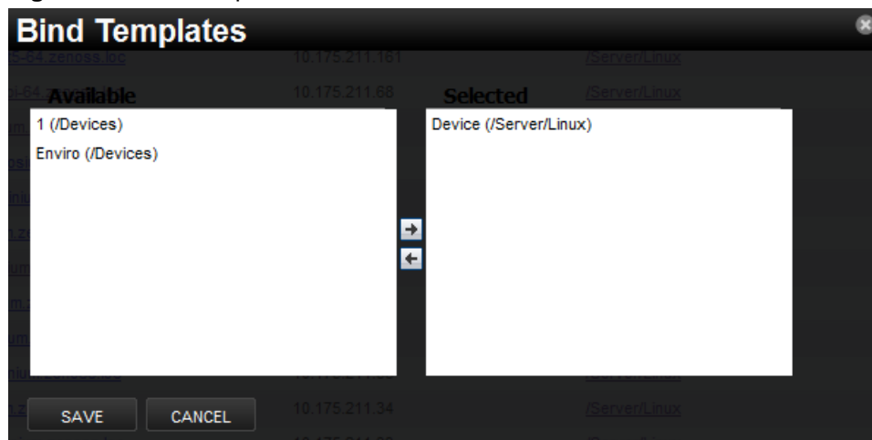
Figure 51: Bind Templates
