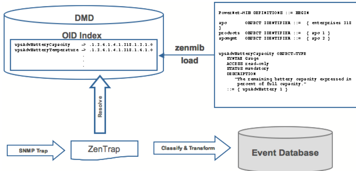
Figure 81: SNMP TRAP transform
