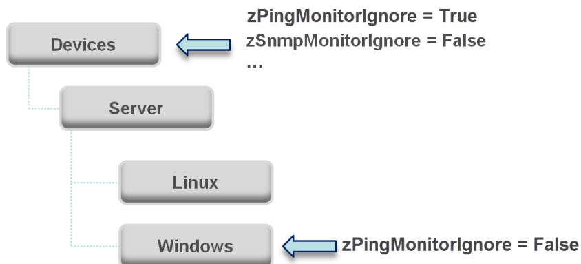
Figure 46: Device class hierarchy - locally defined value (override)
