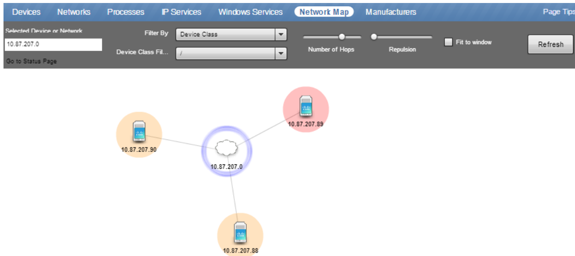
Figure 60: Network Map
