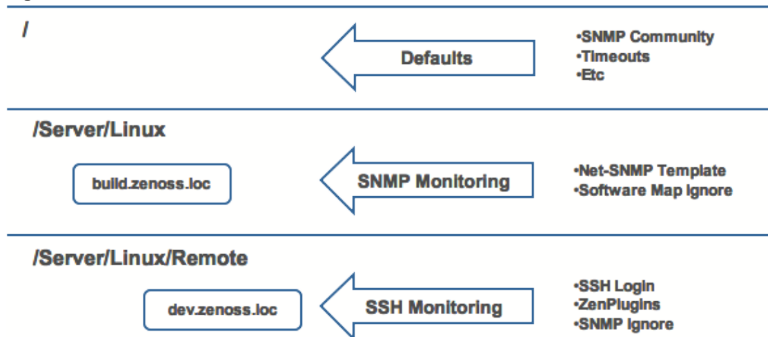
Figure 86: Device class tree and inheritance
