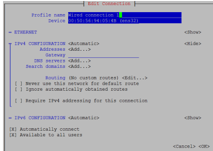
Figure 107: Example: Edit Connection screen
