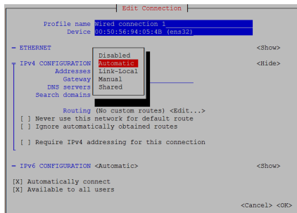
Figure 108: Example: IPv4 Configuration options
