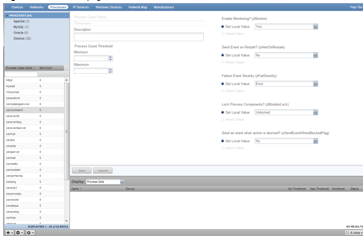
Figure 53: Processes page
