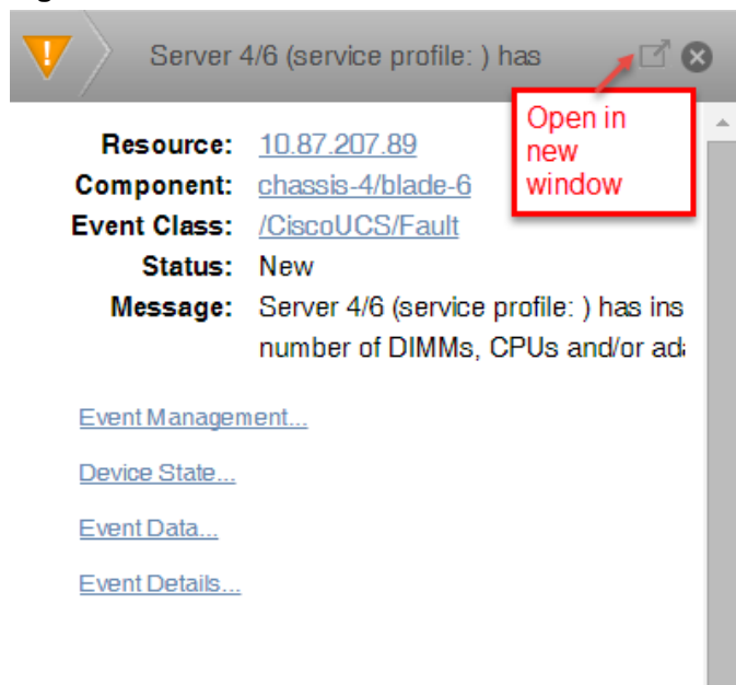
Figure 77: Event details
