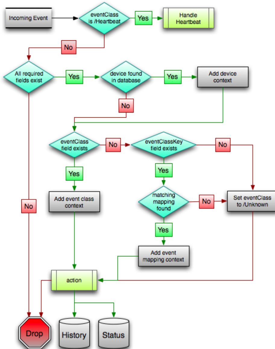
Figure 79: Event processing
