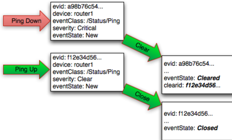
Figure 83: Event Auto-Clear
