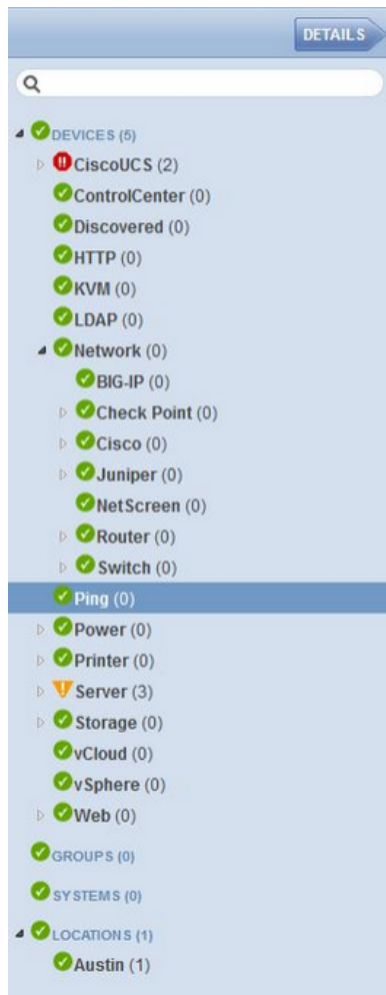
Figure 96: Devices Hierarchy
