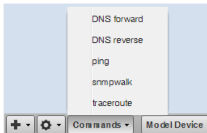
Figure 107: Commands Menu
