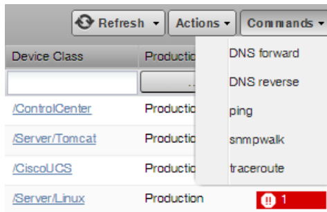
Figure 105: Run Commands
