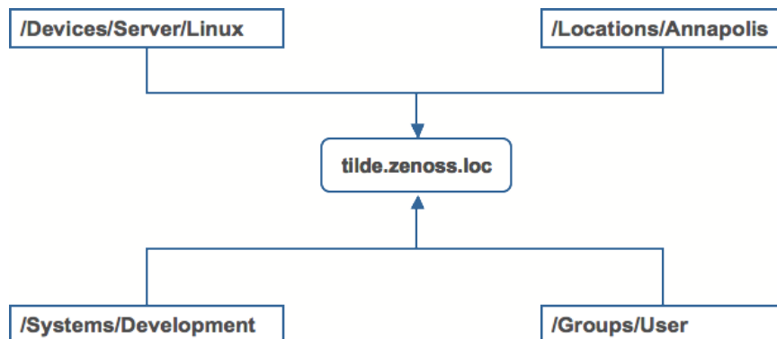
Figure 95: Device Groupings
