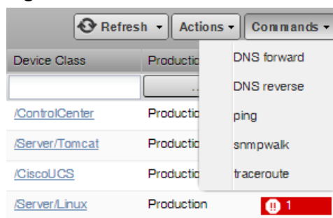
Figure 109: Run Commands
