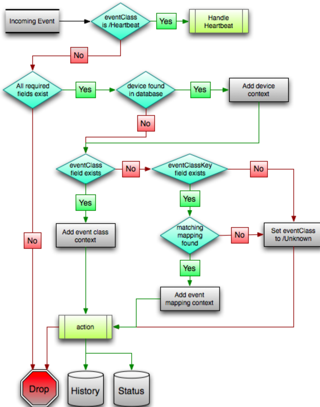
Figure 91: Event Processing
