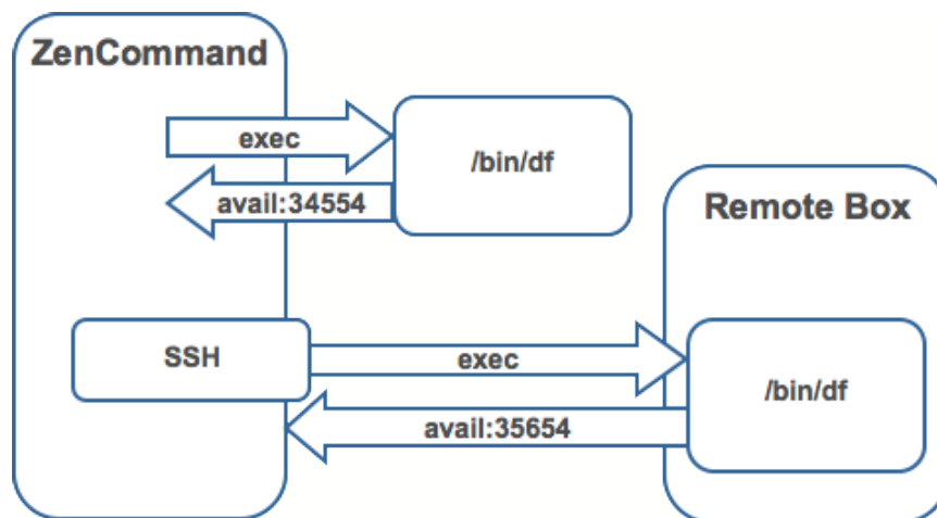
Figure 73: Running ZenCommand
