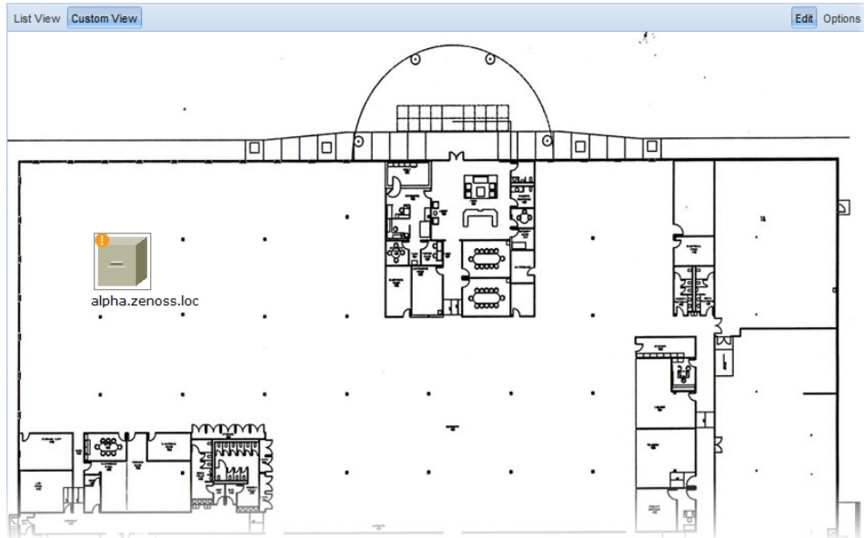
Figure 38: Custom View
