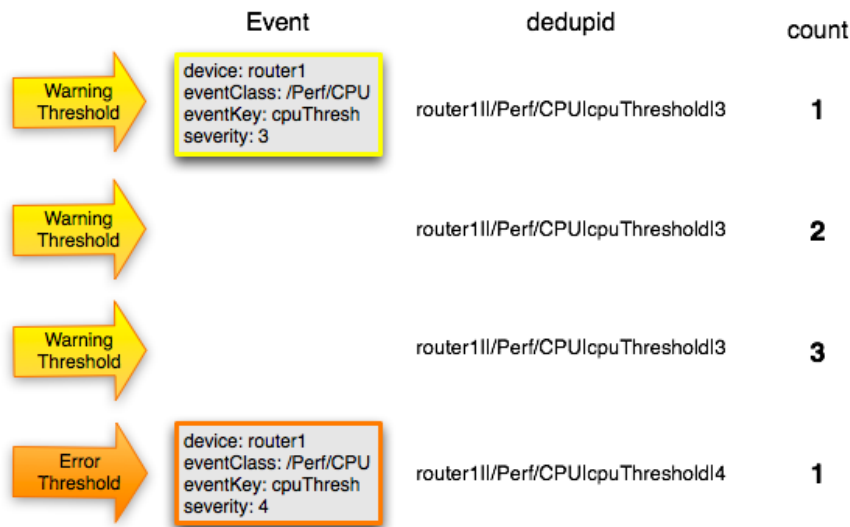
Figure 82: Event De-Duplication
