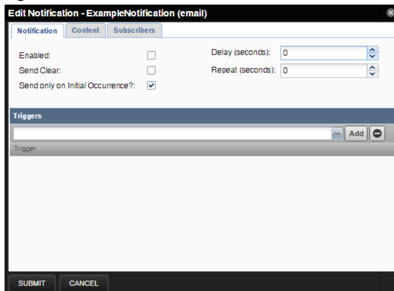
Figure 23: Edit Notification
