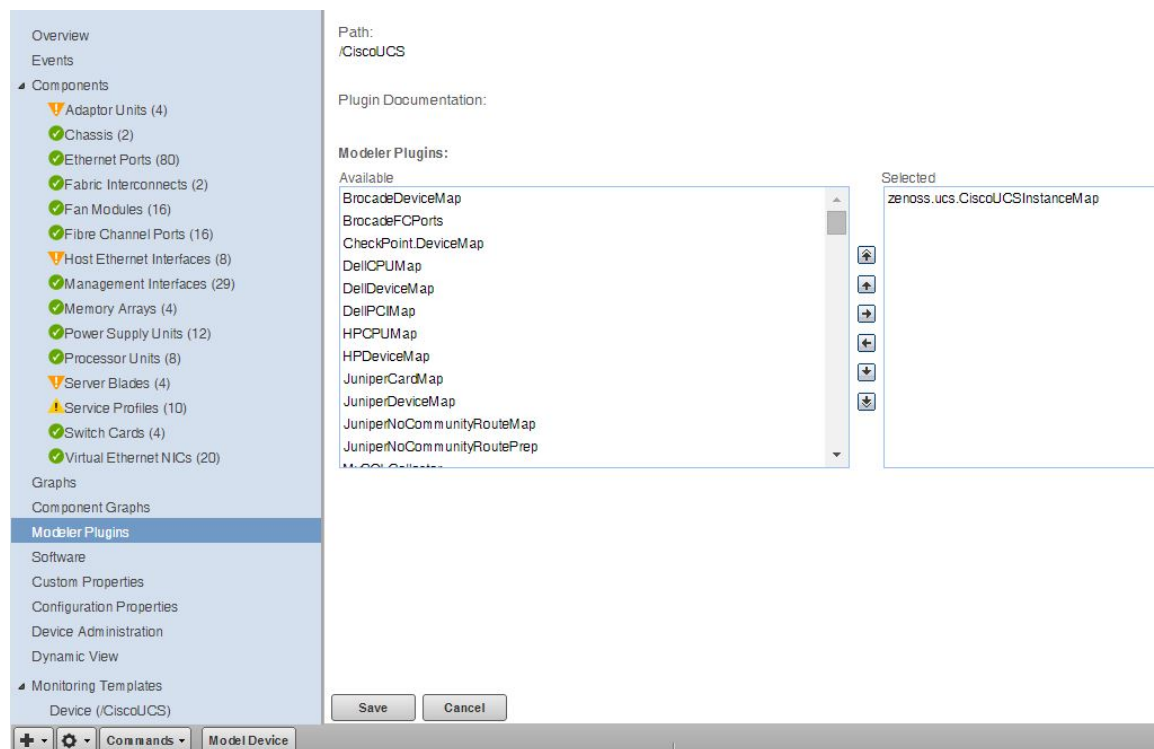
Figure 55: Device (Modeler Plugins)
