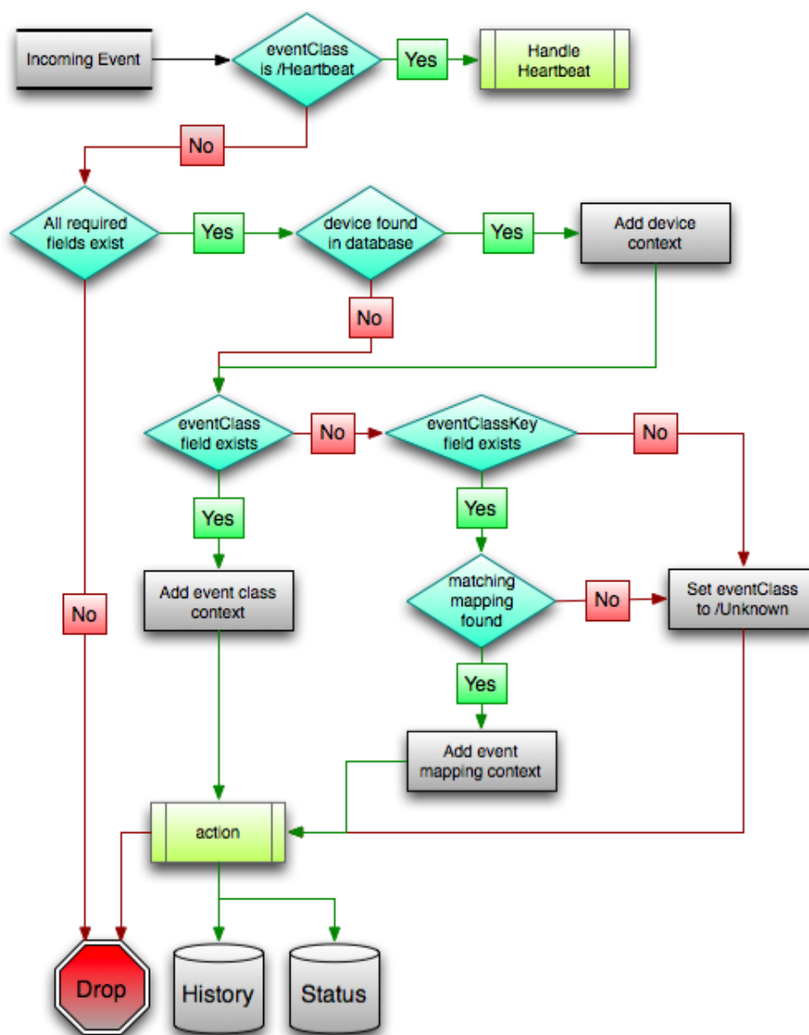
Figure 101: Event Processing
