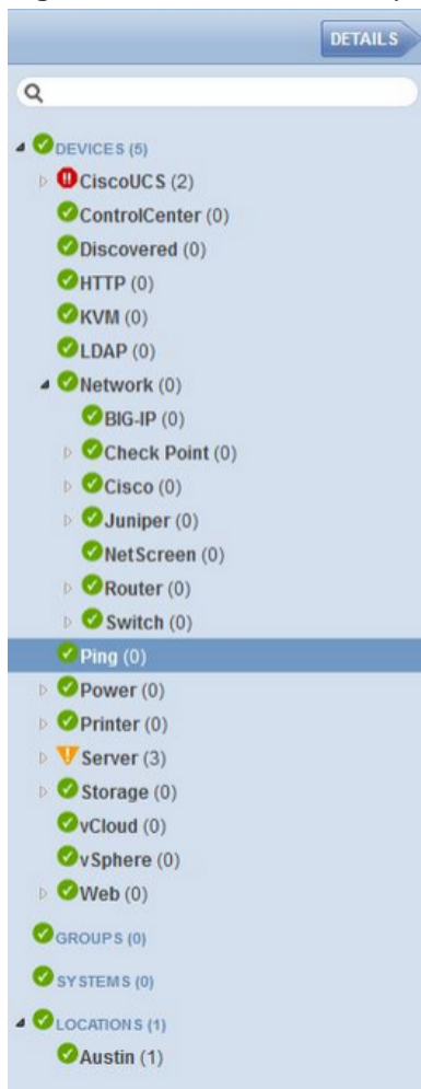
Figure 106: Devices Hierarchy
