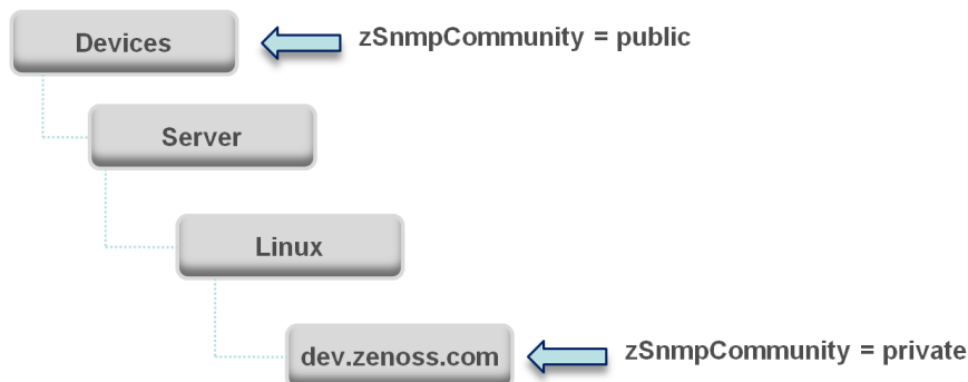
Figure 65: Device Class Hierarchy - Value Set on Device
