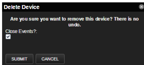
Figure 62: Delete Device
