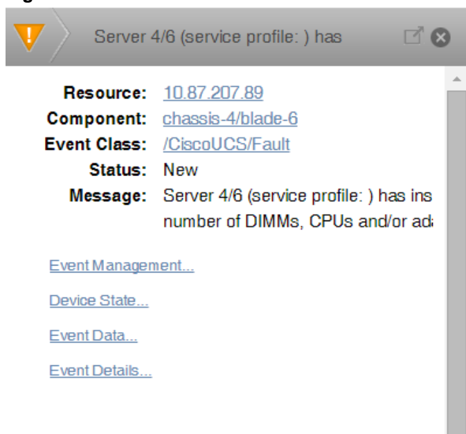
Figure 99: Event Details
