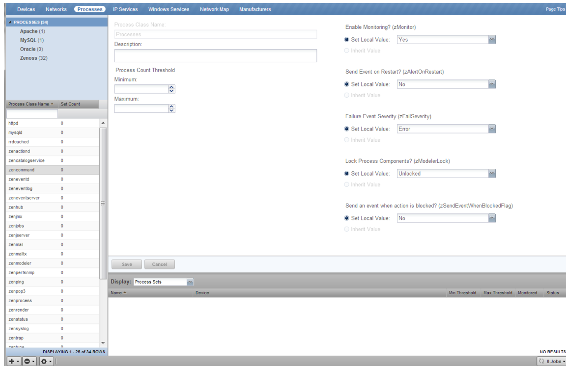
Figure 70: Processes page
