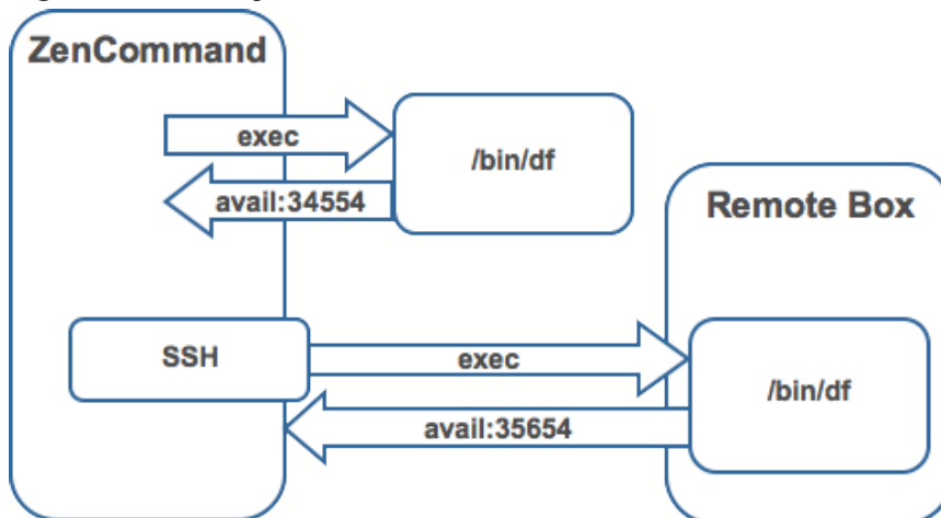
Figure 77: Running ZenCommand
