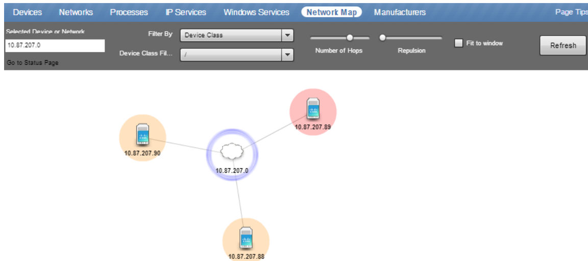
Figure 79: Network Map
