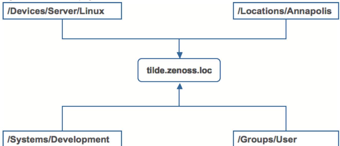
Figure 105: Device Groupings
