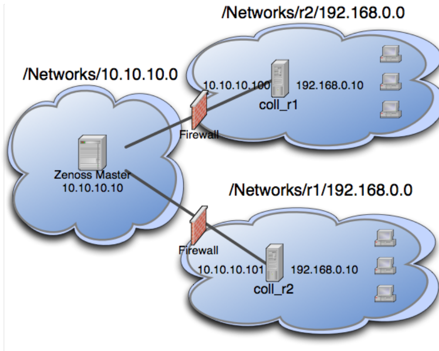
Figure 144: Example IP Realm
