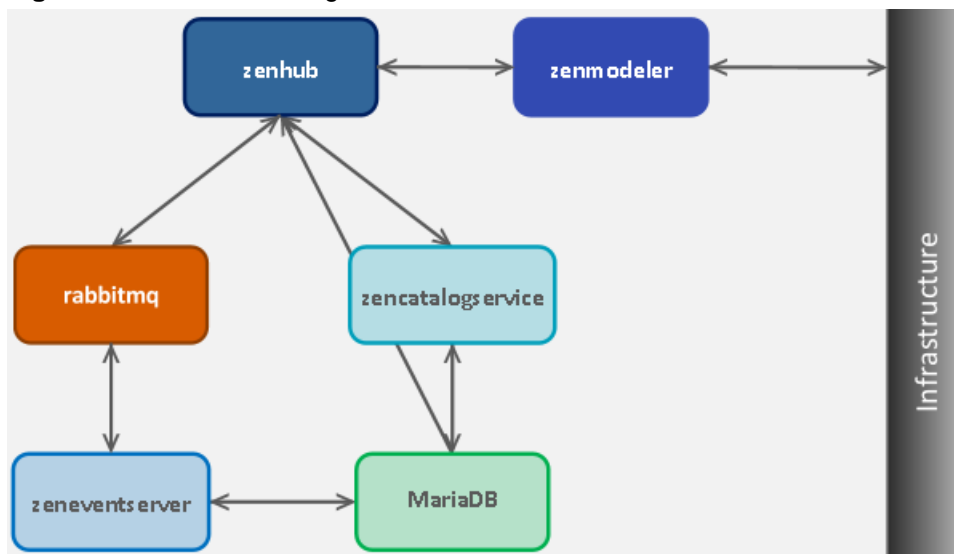
Figure 45: Device Modeling Architecture
