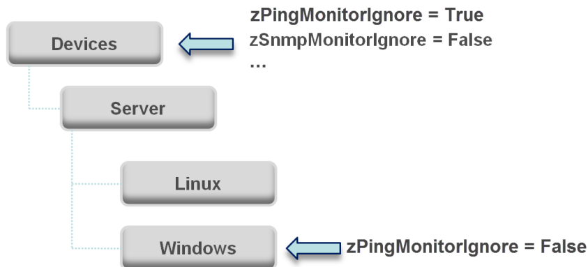
Figure 64: Device Class Hierarchy - Locally Defined Value (Override)
