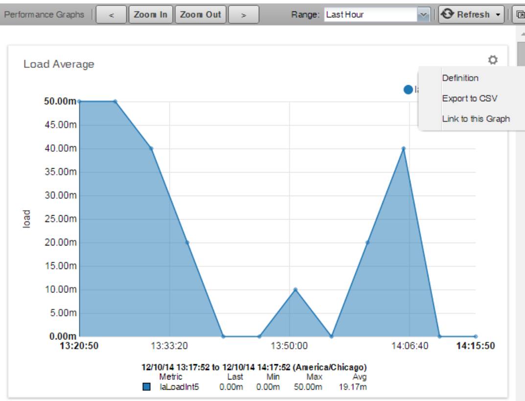
Figure 53: Performance Graph (Device)
