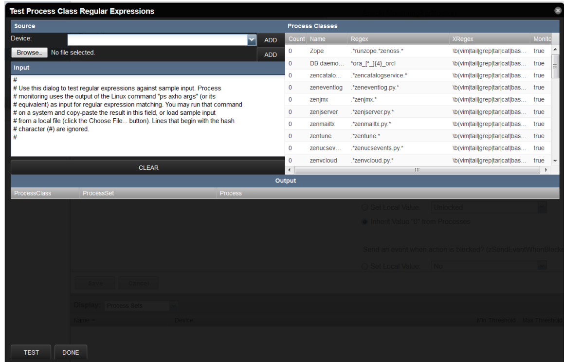
Figure 71: Test all process classes dialog
