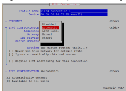
Figure 139: Example: IPv4 Configuration options
