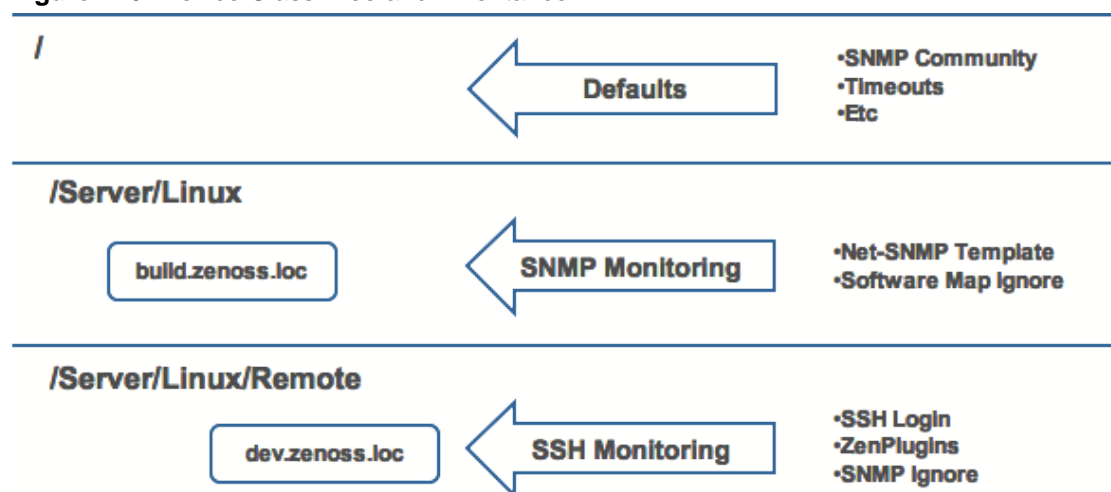
Figure 110: Device Class Tree and Inheritance
