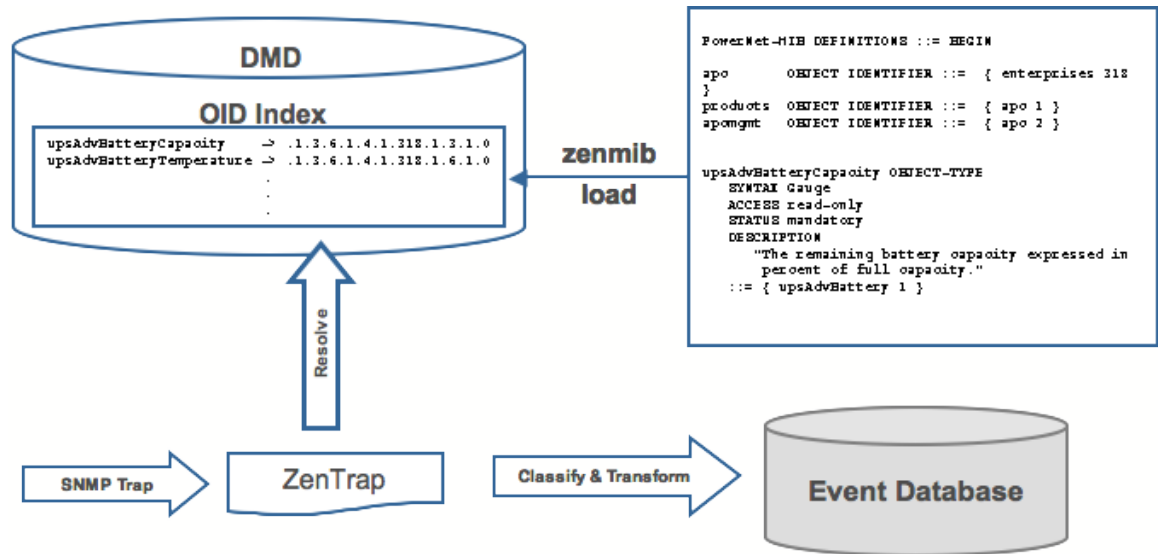
Figure 103: SNMP TRAP Transform
