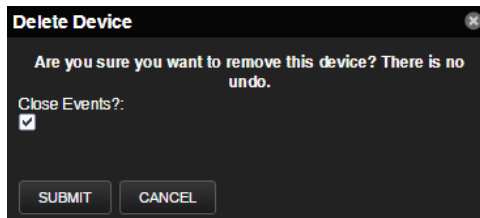
Figure 66: Delete Device
