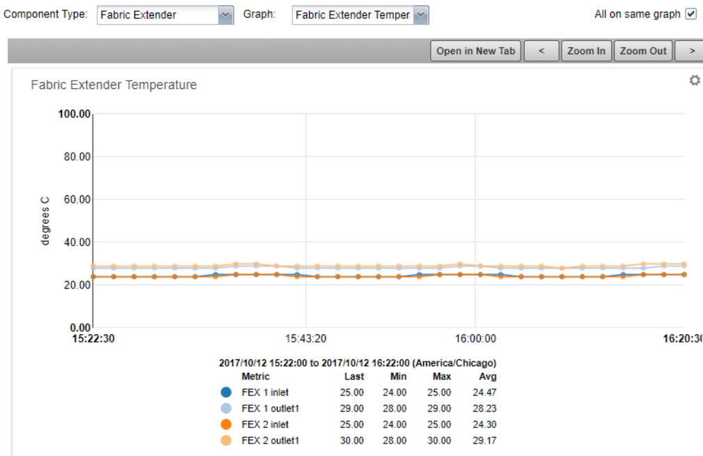
Figure 58: Component graph (Device)
