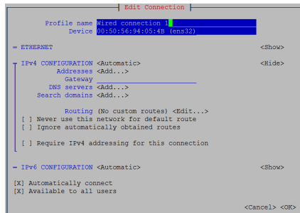
Figure 141: Example: Edit Connection screen
