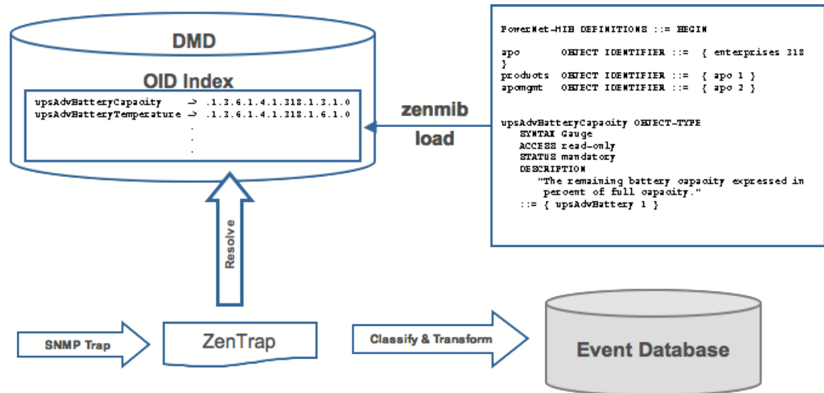
Figure 106: SNMP TRAP transform
