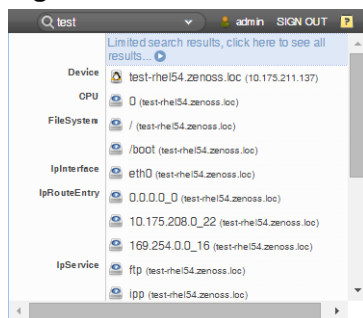
Figure 10: Search Results
