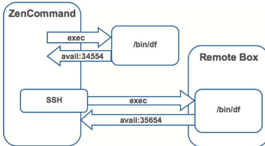
Figure 80: Running ZenCommand
