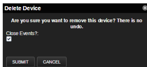
Figure 65: Delete Device
