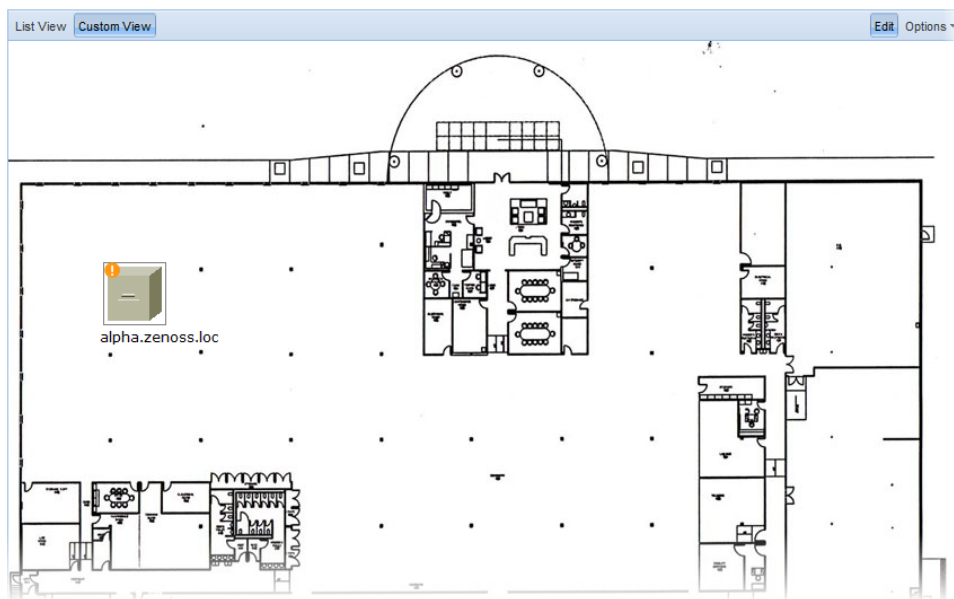
Figure 38: Custom view
