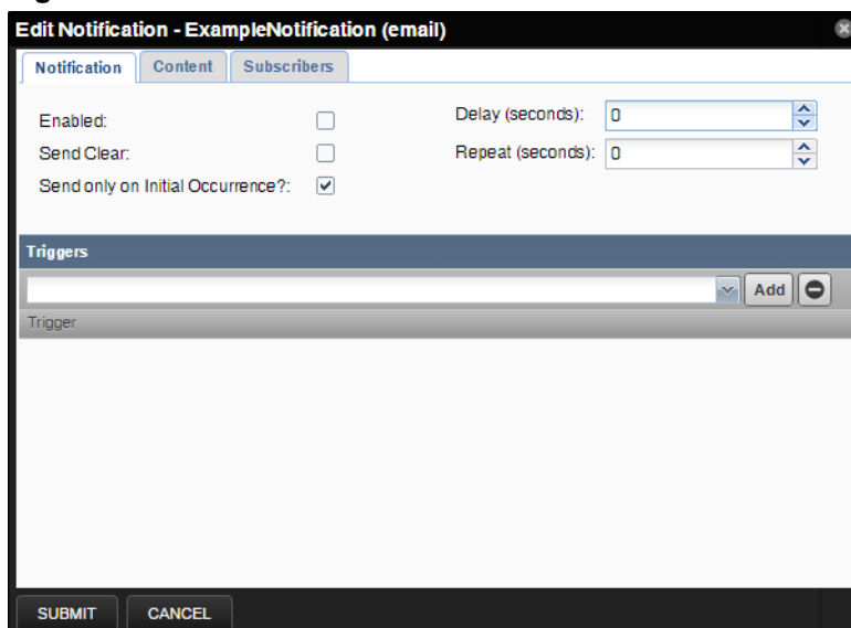
Figure 23: Edit Notification
