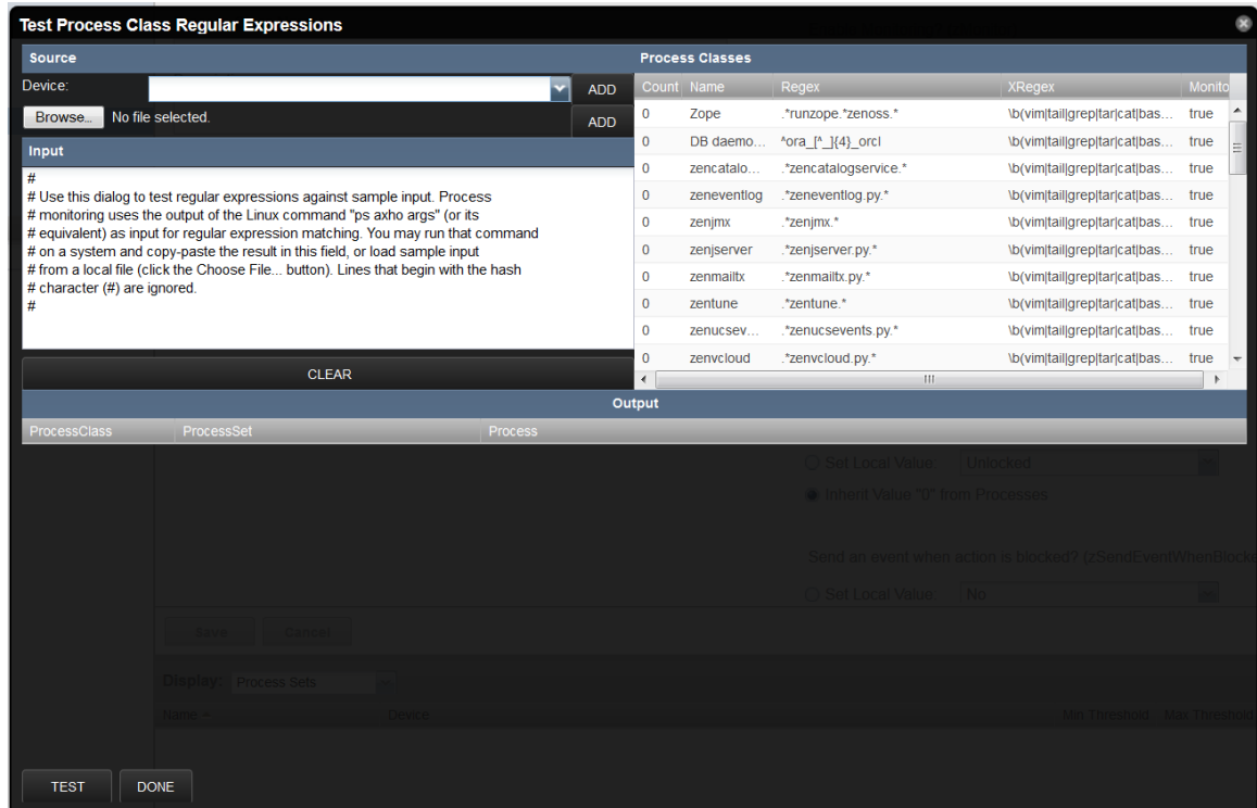
Figure 74: Test all process classes dialog
