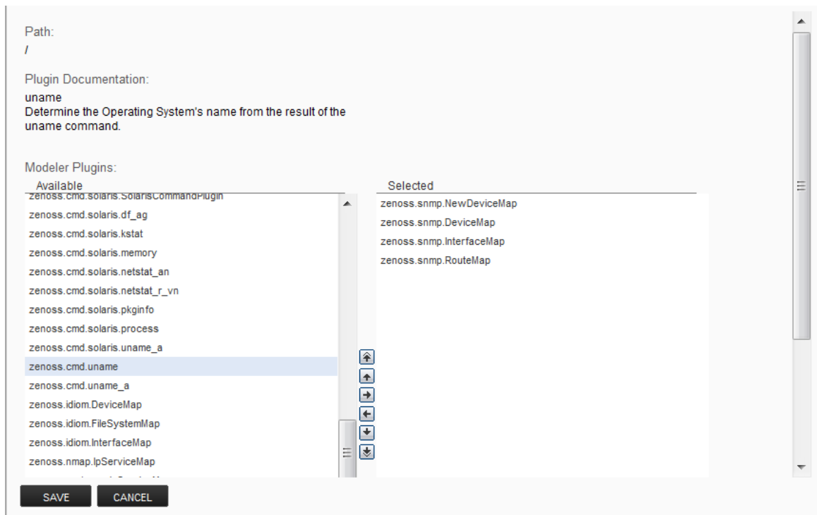
Figure 48: Add plugin
