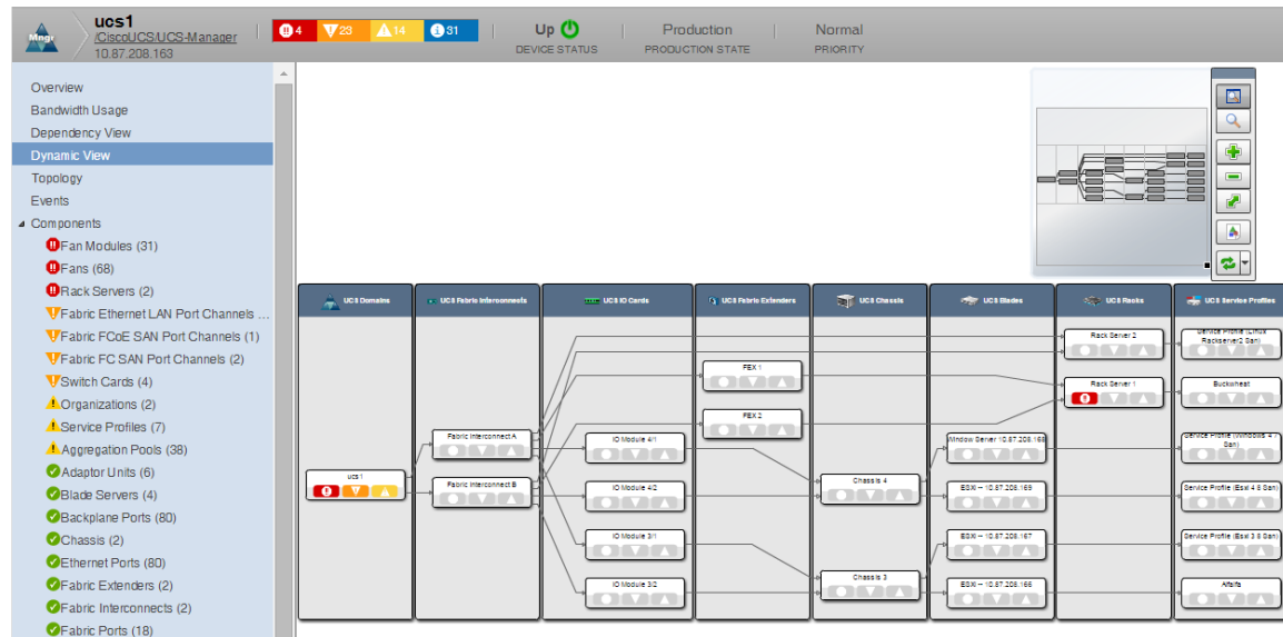
Figure 52: Dynamic view
