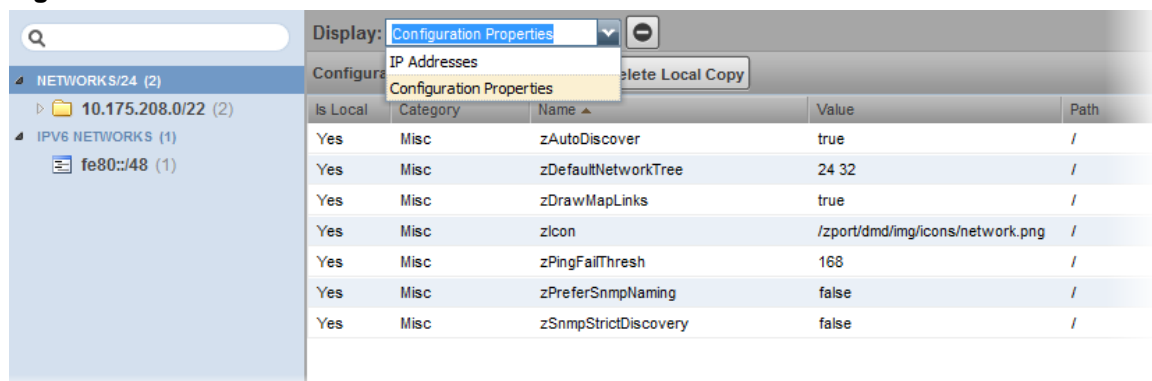
Figure 71: Networks
