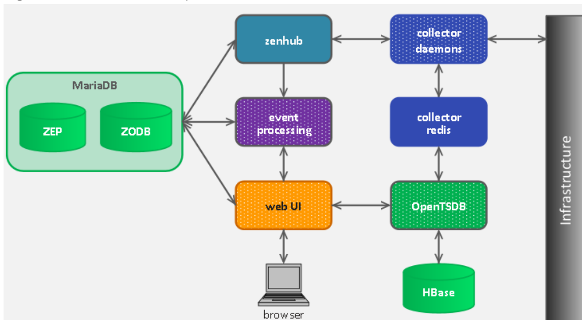
Figure 82: Data collection simplified architecture
