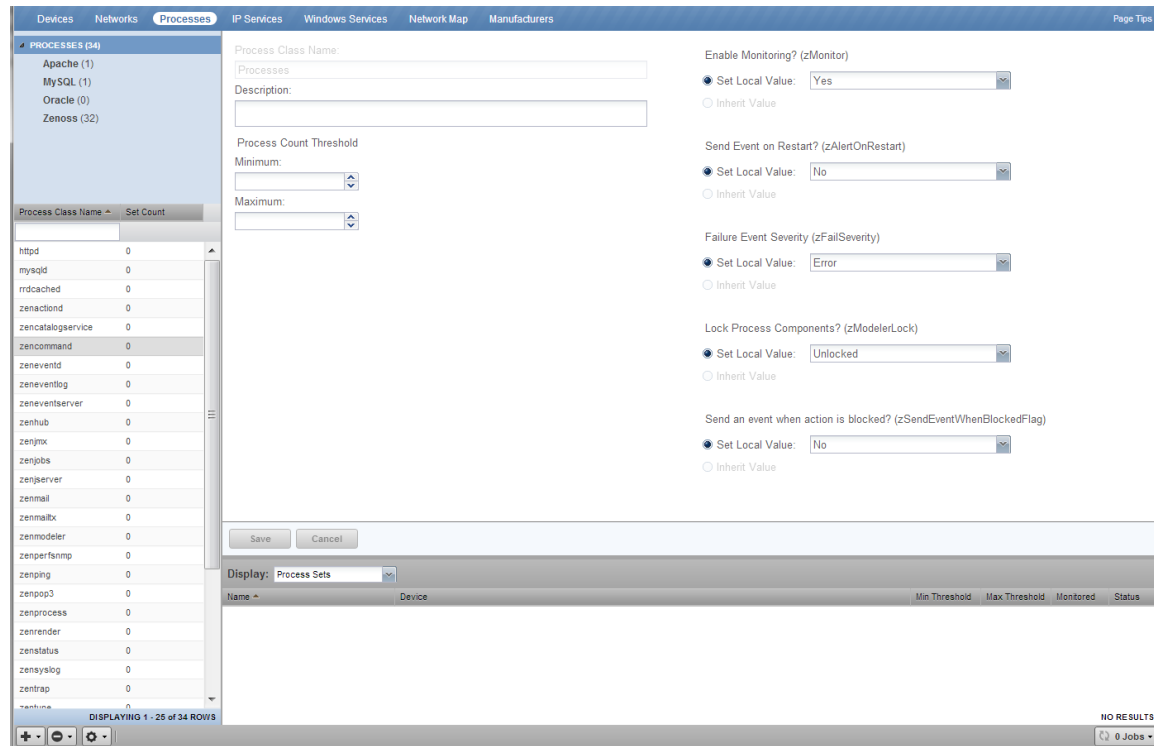
Figure 73: Processes page
