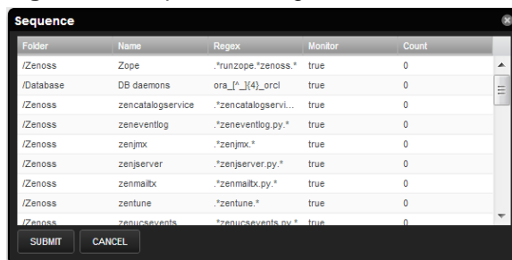
Figure 77: Sequence dialog
