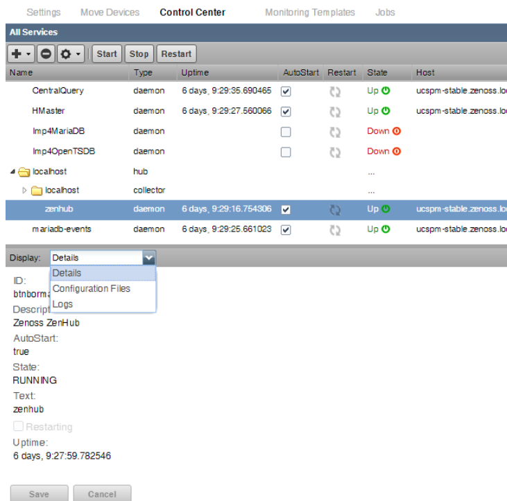
Figure 116: Control Center - daemon details
