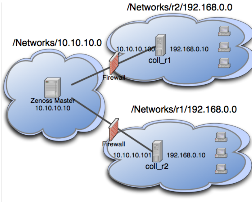
Figure 146: Example IP realm
