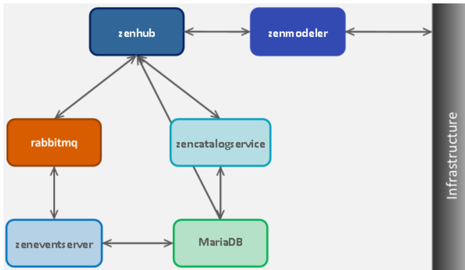
Figure 48: Device modeling architecture
