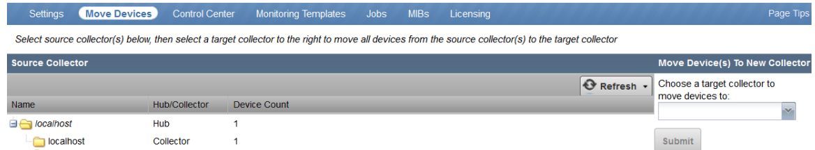
Figure 117: Move Devices
