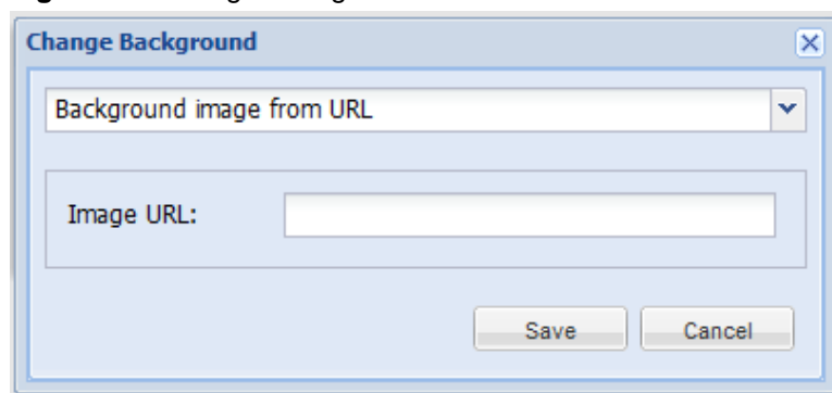
Figure 40: Change Background
