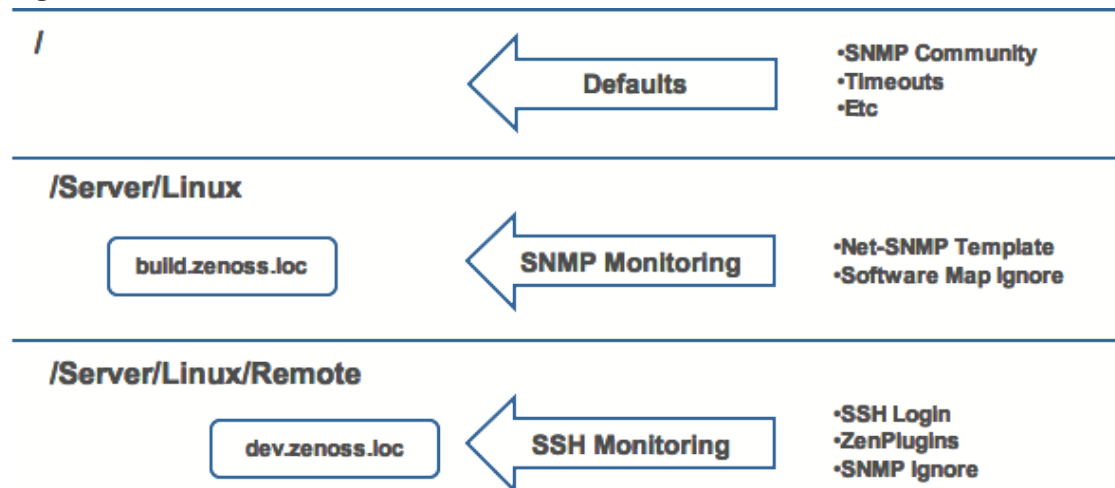
Figure 113: Device class tree and inheritance
