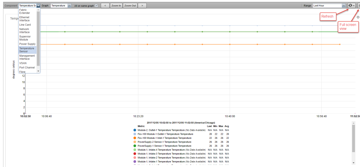
Figure 58: Component graph (Device)
