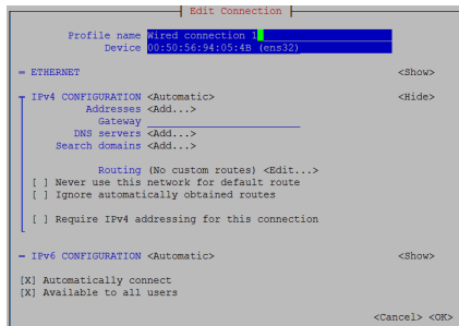
Figure 140: Example: Edit Connection screen
