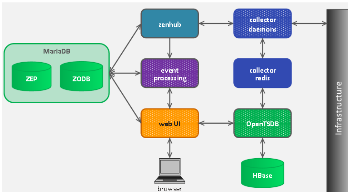
Figure 83: Data collection simplified architecture
