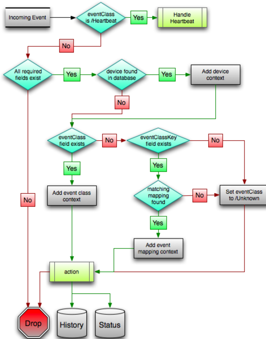
Figure 104: Event processing
