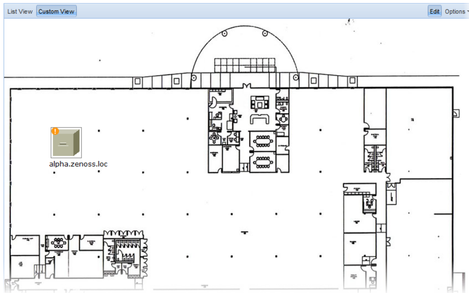
Figure 40: Custom view
