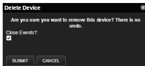
Figure 68: Delete Device
