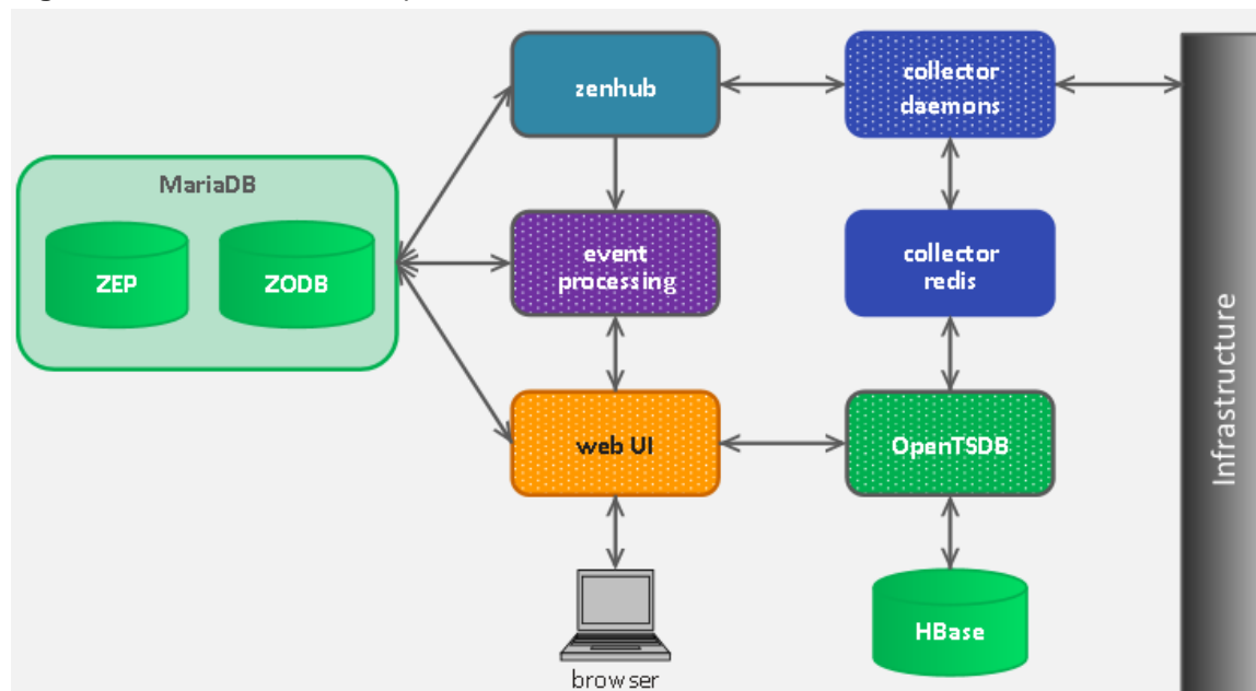
Figure 85: Data collection simplified architecture
