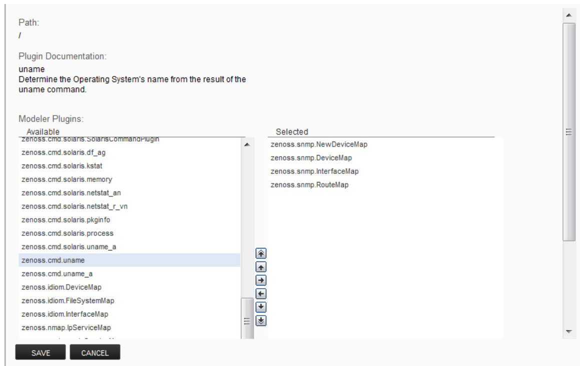
Figure 51: Add plugin
