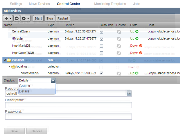
Figure 119: Control Center - hub details
