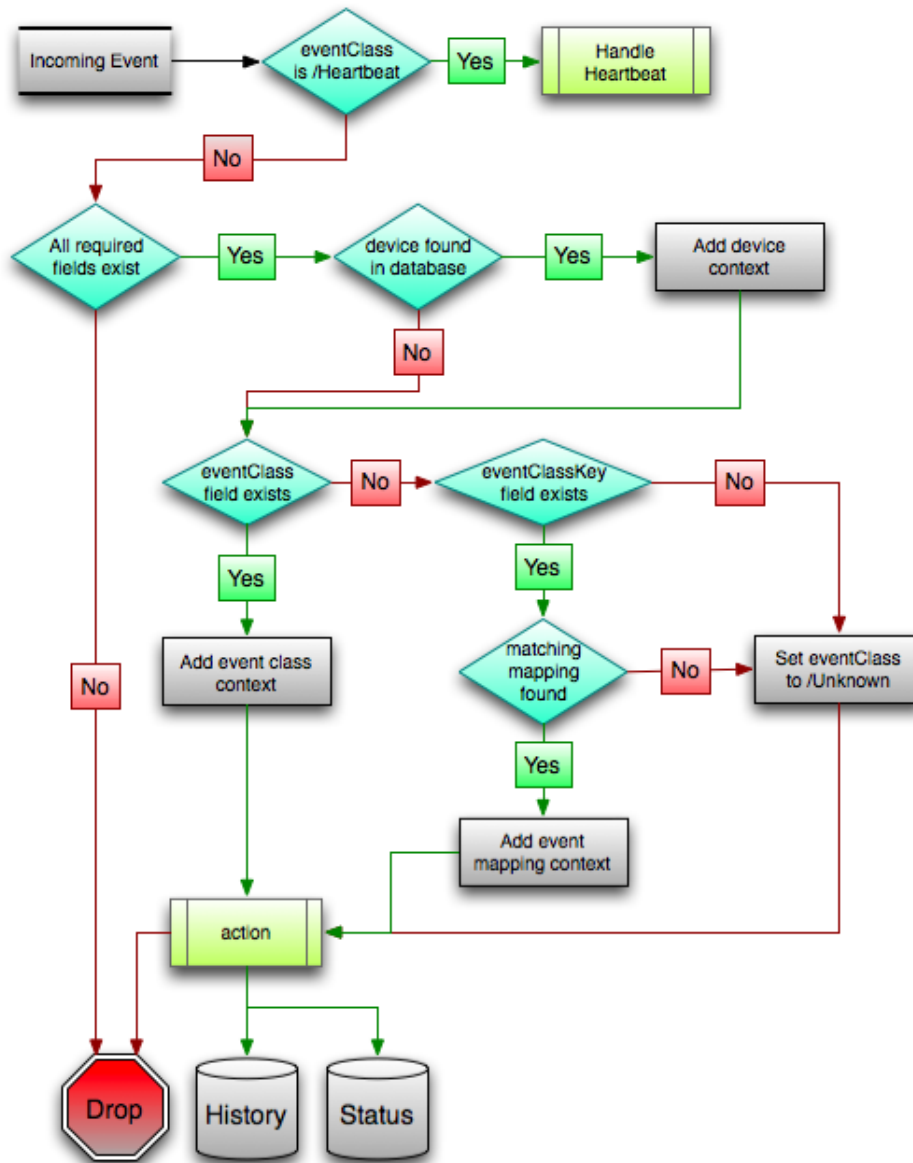
Figure 109: Event processing
