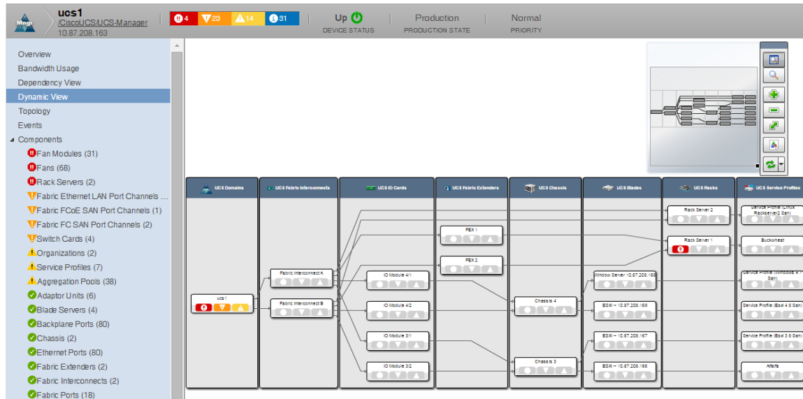
Figure 55: Dynamic view
