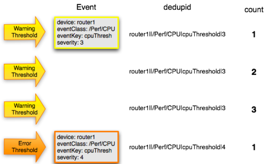
Figure 100: Event de-duplication
