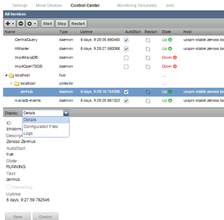
Figure 120: Control Center - daemon details
