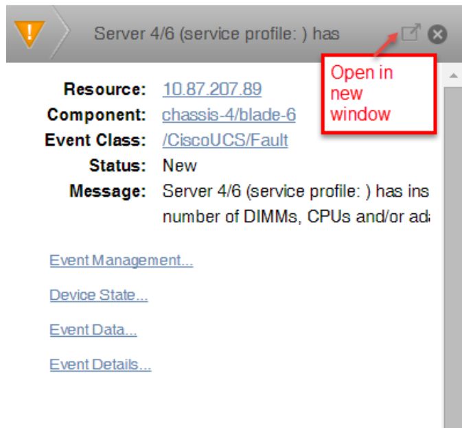
Figure 107: Event details
