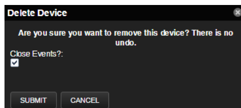
Figure 68: Delete Device
