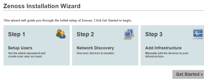
Figure 1: Setup Wizard
