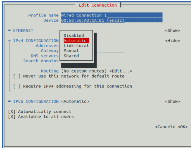
Figure 22: Example: IPv4 Configuration options
