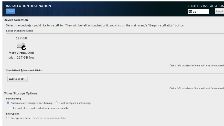
Figure 18: INSTALLATION DESTINATION page
