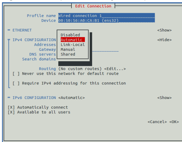
Figure 10: Example: IPv4 Configuration options
