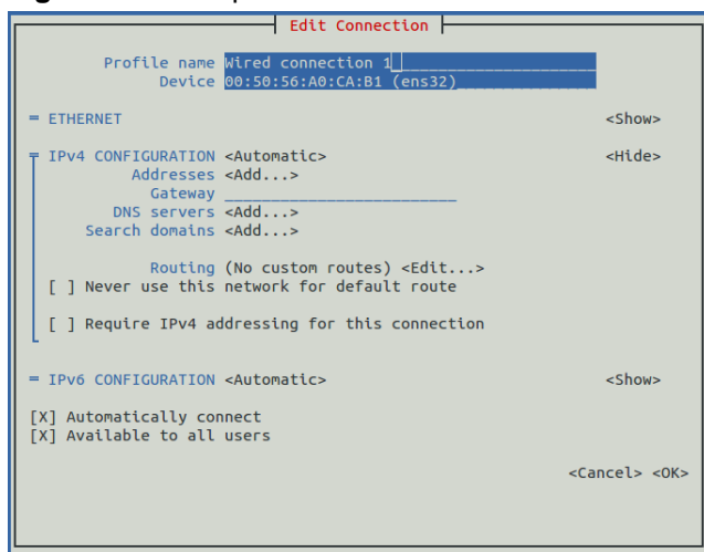
Figure 21: Example: Edit Connection screen
