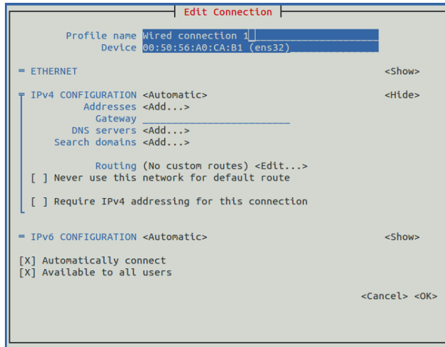
Figure 9: Example: Edit Connection screen
