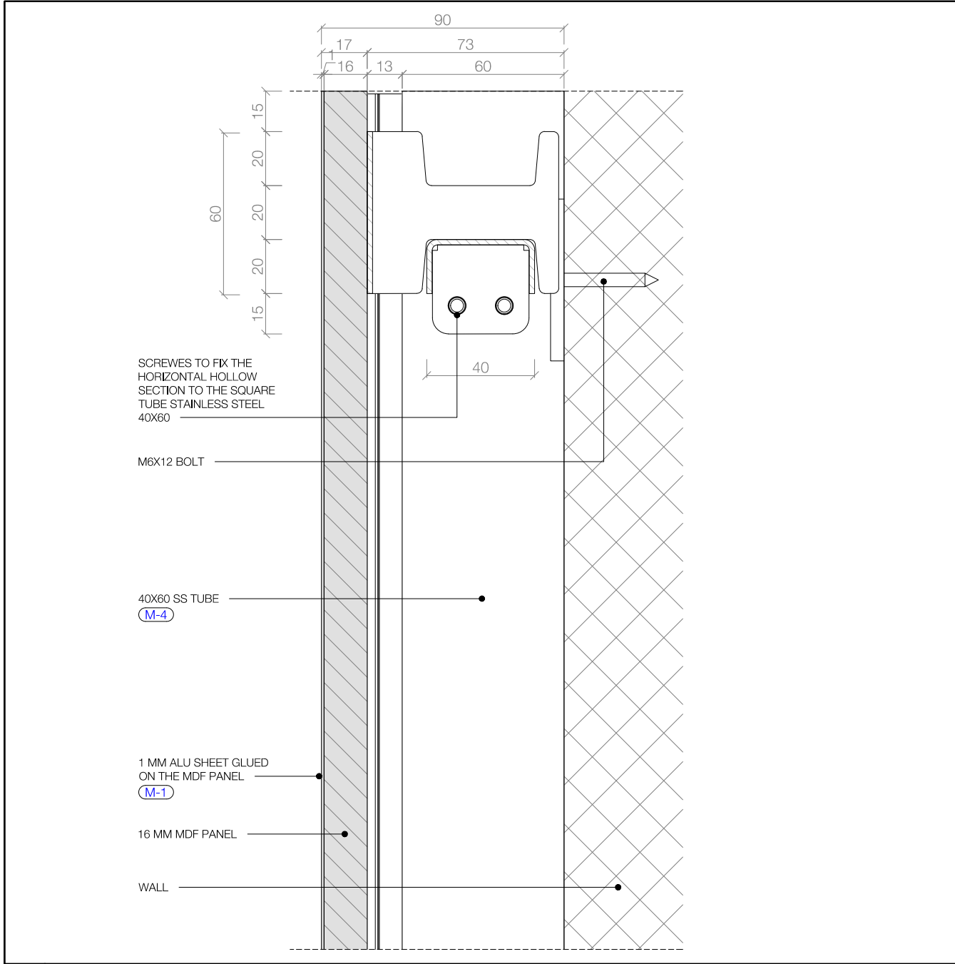
2 DETAIL SECTION TOP SINGLE PANEL 1:2 @ A3
