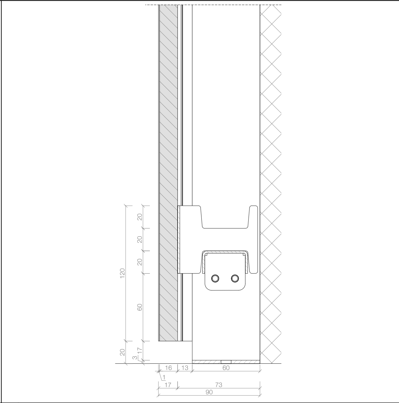
4 DETAIL BOTTOM STRUCTURE 1:2 @ A3
