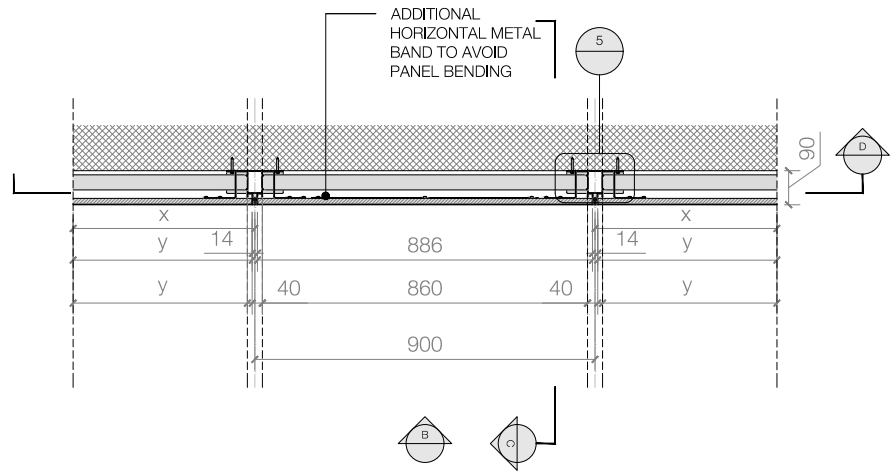
A PLAN 1:20 @ A3
