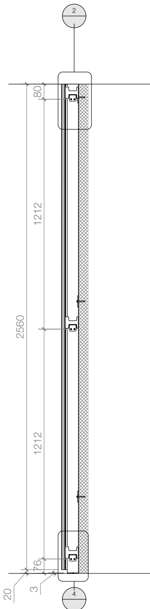
1 DETAIL 1:2 @ A3
