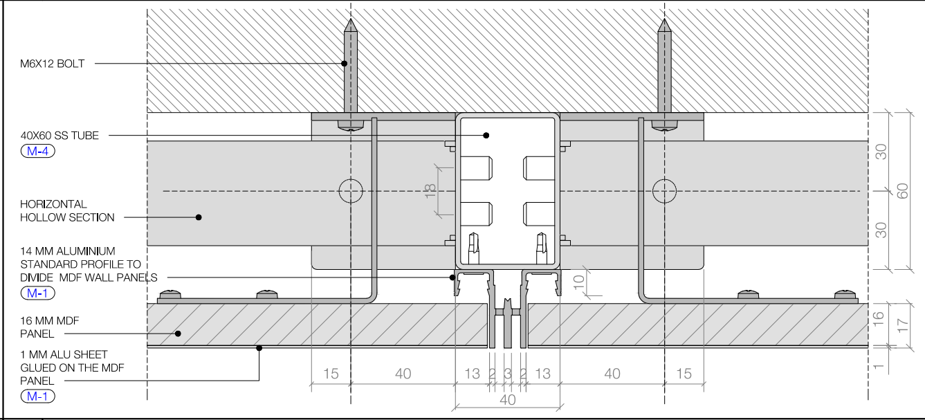
5 DETAIL ALU PROFILE 1:2 @ A3
