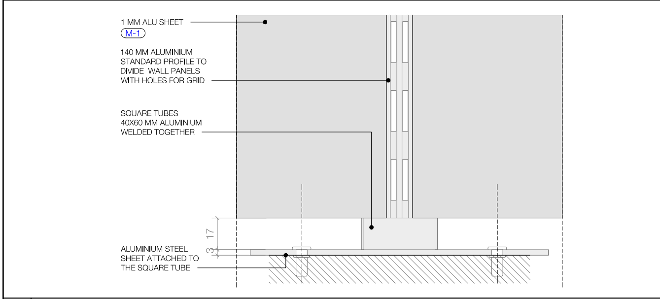
3 DETAIL BOTTOM PANEL COVERING 1:2 @ A3
