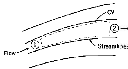
Fig. 6.5 Flow through a stream tube.
