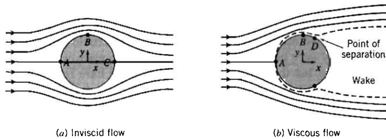
Fig. 2.12 Qualitative picture of incompressible flow over a sphere.
