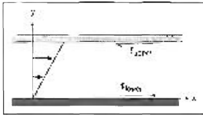
(e) Directions of shear stresses on upper and lower plates.
