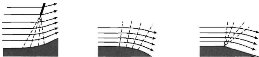
(a) Isentropic compression waves
