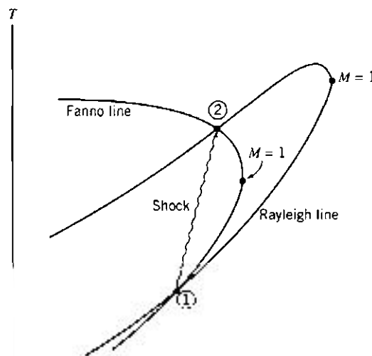
Fig. 12.18 Intersection of Fanno line and Rayleigh line as a solution of the normal-shock equations.
