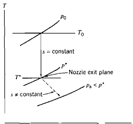
Fig. 12.7 Schematic Ts diagram for choked flow through a converging nozzle.
