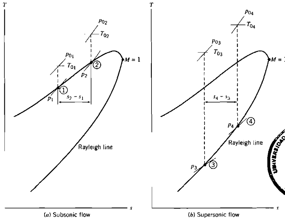
Fig. 12.16 Reduction in stagnation pressure due to heat addition for two flow cases.
