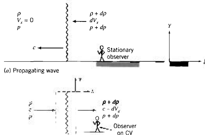
(a) Propagating wave (b) Inertial control volume moving with wave, velocity c Fig. 11.1 Propagating sound wave showing control volume chosen for analysis.
